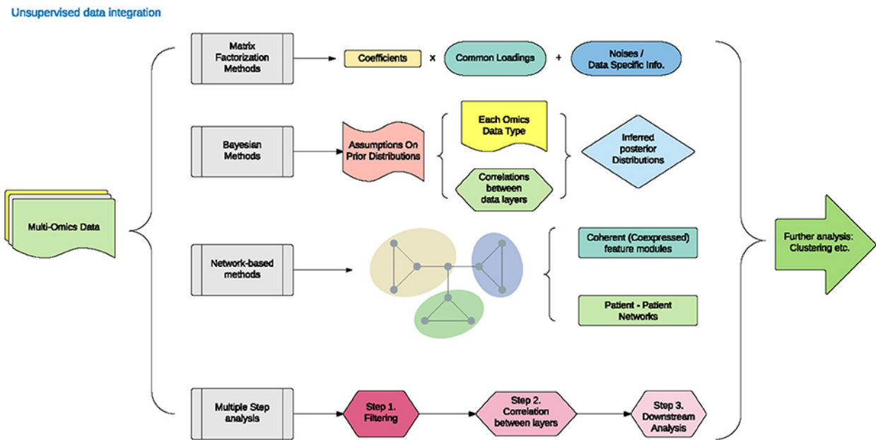
Figure 1.3. Unsupervised data integration methodology. Adapted from figure 1 from Huang 2017.
