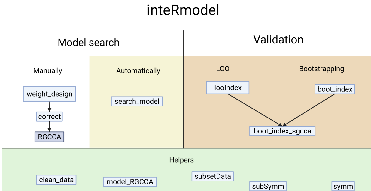
Figure 4.2. ‘inteRmodel’ functions and workflow. Functions provided by the inteRmodel package to help on the process, search and validate models of relationships using RGCCA . Created with BioRender.com
