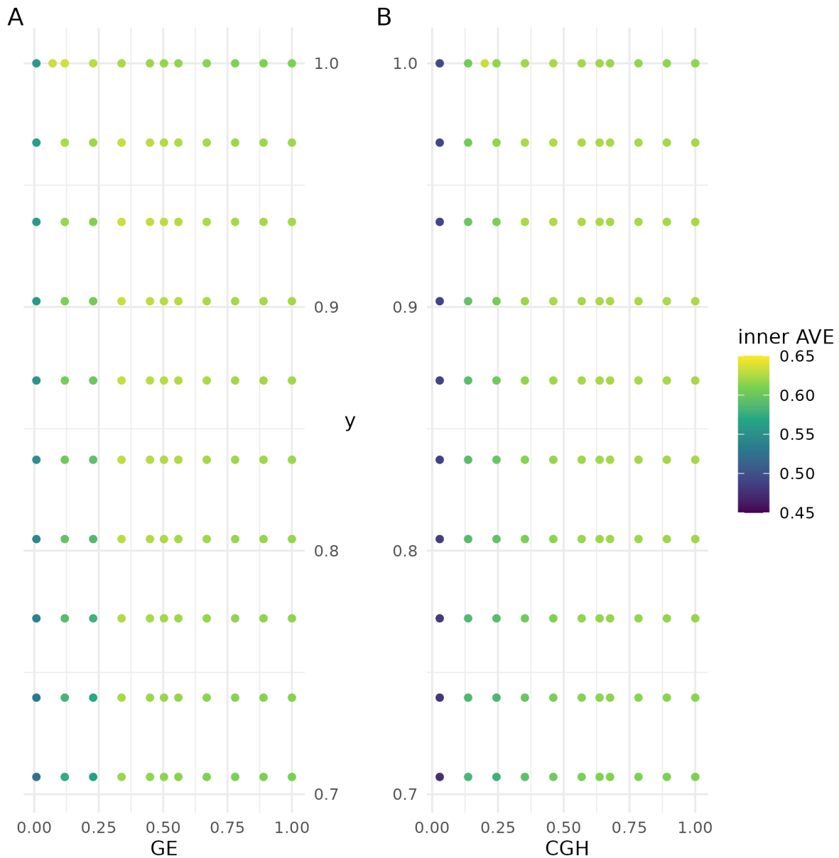
Figure 4.3. Effect of tau on the inner AVE in the Puget dataset. The suggested tau value is the column between the regular grid, on the ordinate axis the y 's tau values and on the abscissa the gene expression (GE) on the left and the comparative genomic hybridization (CGH) on the right. The highest inner AVE is with high tau values for y and middle to upper values for GE and CGH.
