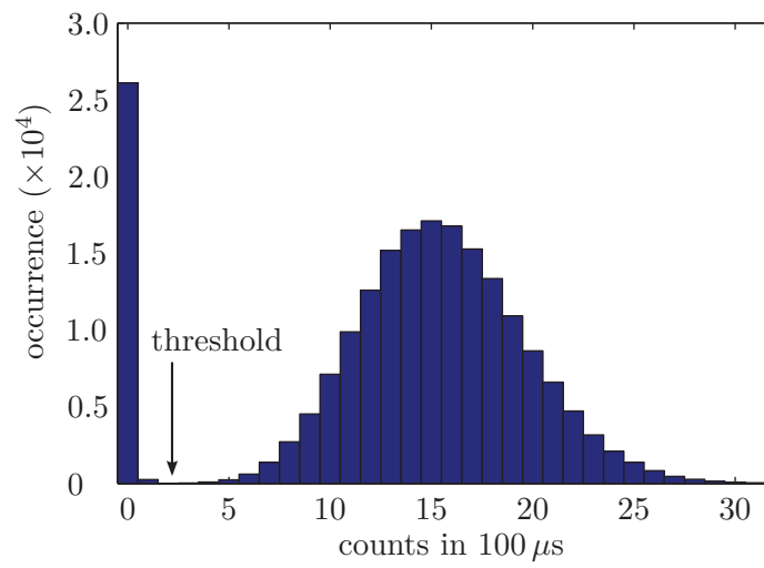
Figure 4.16.: Measured histogram of 397 nm fluorescence photons during the detection phase of the sequence. The displayed data correspond to an acquisition time in part IV of the sequence of 100 \mu\text{s} with a continuous countrate of 1.55 \cdot 10^5 \text{ s}^{-1} for the ion being in the S_{1/2} state and 100 \text{ s}^{-1} for the ion being in D_{5/2} . The optimal threshold to distinguish between the two states in a single measurement is at 2.
