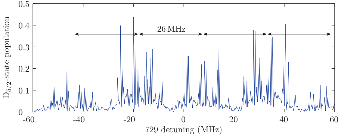
Figure 4.20.: 729 spectrum of single ion trapped in the DT, without optical pumping. Strong sidebands at the trap radio frequency of 26 MHz due to micro motion of the ion are visible, making the spectrum appear multiple times.
