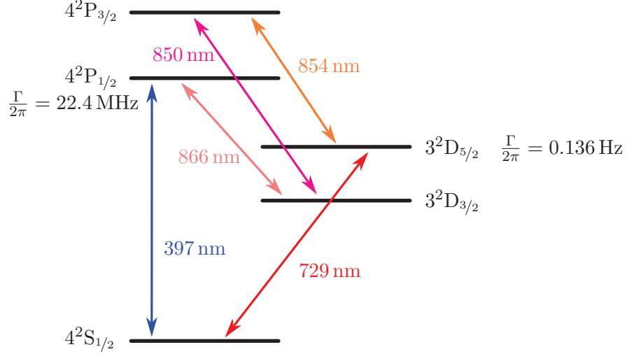
Figure 1.2.: Level scheme of ^{40}\text{Ca}^+ with all optical transitions that are experimentally accessible with lasers in the current set-up. The indicated decay rates \Gamma of the P_{1/2} and D_{5/2} state are taken from [83, 84].
