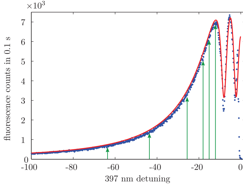
Figure 5.3.: 397 nm spectroscopy with the repumper at 866 nm on resonance and laser powers of 4 \mu\text{W} for the blue and 16 \mu\text{W} for the red beam. Close to resonance of the 397 the ion starts heating and the fluorescence signal drops. The red curve is a simulation of the expected spectrum for the used laser parameters with the calibration obtained by the previously shown 866 nm spectrum. The green arrows indicate the 397 detunings for which the cooling dynamics were investigated in detail.
