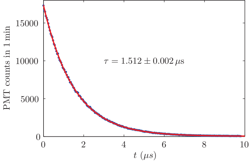
Figure 3.12.: Decay of combined 397 nm and 393 nm fluorescence during part II of the single-photon sequence caused by transfer of population to the D_{5/2} state. The data are displayed with 40 ns bin size for a sequence repetition rate of 70 kHz. The red curve is an exponential fit to determine the decay constant.
