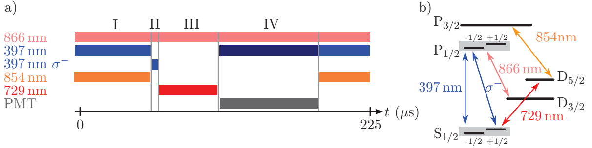
Figure 4.15.: a) Typical timing of the laser sequence that is used for 729 nm spectroscopy. Details are given in the text. Depending on the experiment, the 729 pulse in part III varies in length or gets replaced by a sequence of several pulses. b) Level scheme for ^{40}\text{Ca}^+ with all relevant transitions.
