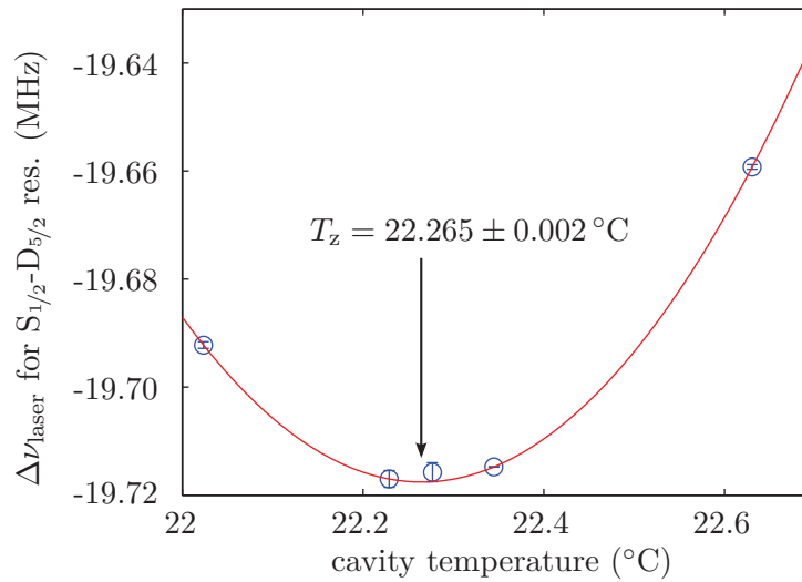
Figure 4.23.: Precise measurement of T_z . The data points are the AOM detunings of the 729 laser to be on resonance with the center of the S_{1/2} - D_{5/2} transition. The red curve is a parabolic fit.
