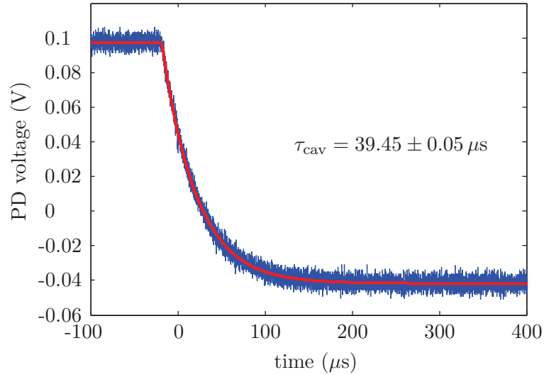
Figure 4.13.: Cavity ring-down measurement with a fast photodiode (PD). The red curve shows an exponential fit to the data. From ten individual ring-down measurements a cavity-field decay time of \tau = 39.45 \pm 0.05 \mu\text{s} is derived.
