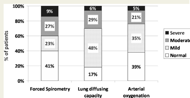
Figure 2 Distribution of the severity of abnormalities found in forced spirometry, lung diffusing capacity ( DL_{CO} ) and arterial oxygenation ( PaO_2 ). The severity of spirometric abnormalities was graded according to the FEV_1 value (obstructive; mild \geq 80\% ; moderate 50–79%; severe 30–49%; or very severe < 30\% ) for obstructive ventilatory defects and/or TLC values (mild 70–80%; moderate 50–69%; severe 40–49%; or very severe < 40\% ) for restrictive ones. Impairment of DL_{CO} was graded as mild (60–80% reference), moderate (40–59% reference) or severe ( < 40\% reference). Arterial hypoxaemia ( PaO_2 \leq 80 mmHg) was graded as mild ( PaO_2 70–80 mmHg), moderate ( PaO_2 60–69 mmHg) or severe ( PaO_2 40–59 mmHg). For further explanations, see text.
