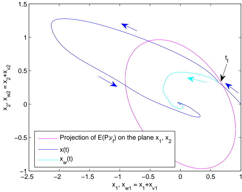
FIGURE 9.5: Phase plane of x(t) and x_w(t) , t_f = t_I = 0.5 s.
