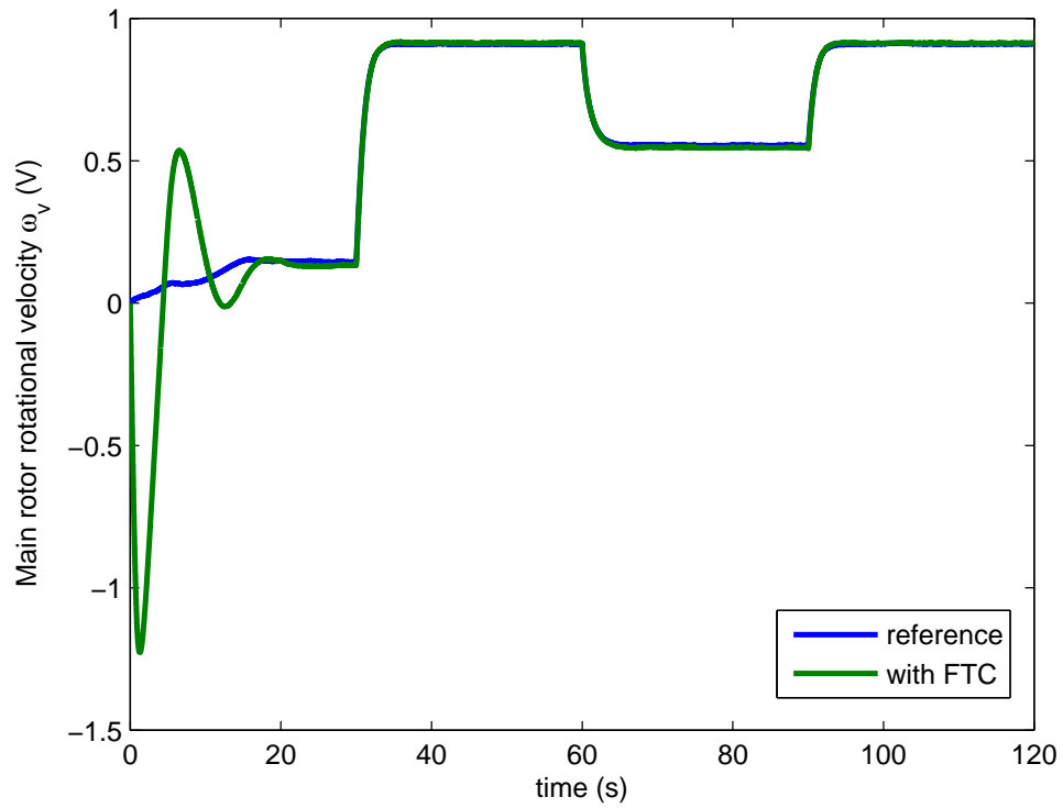
FIGURE 8.13: Faulty main rotor response (comparison between TRMS and reference model states, with FTC).
