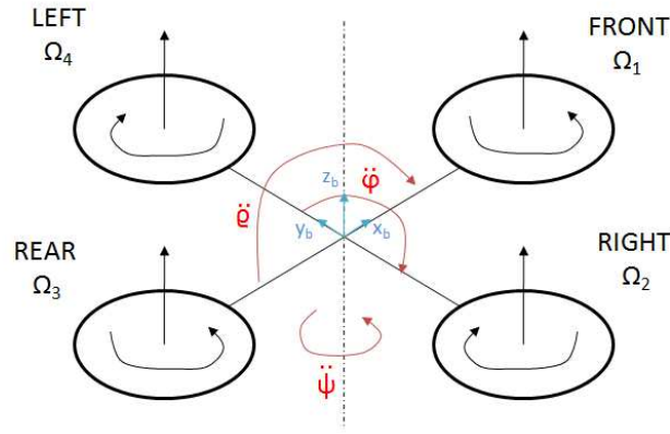
FIGURE 7.1: Quadrotor scheme.
