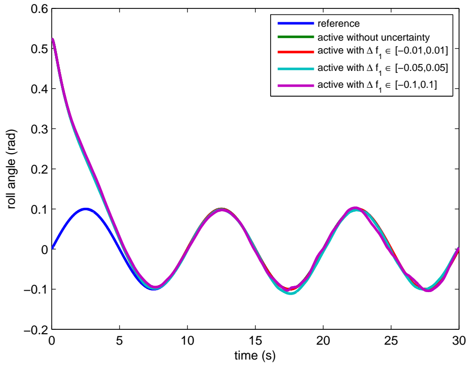
FIGURE 7.6: Roll angle response (active FTC without and with uncertainty, f_1 = 0.7 ).
