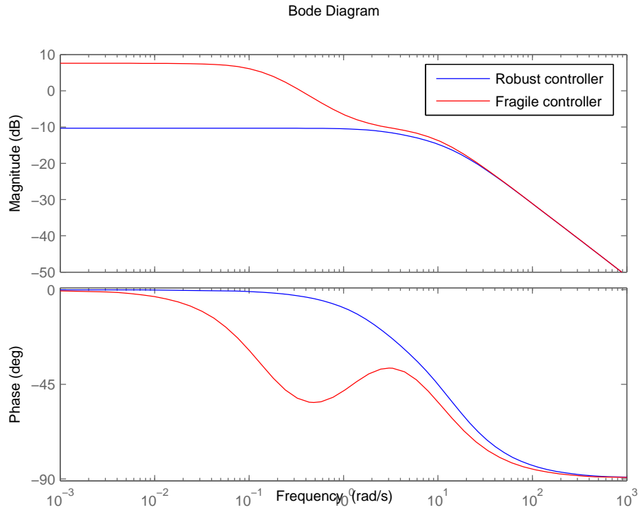
FIGURE 4.6: Robust \mathcal{H}_\infty performance: Bode plot
