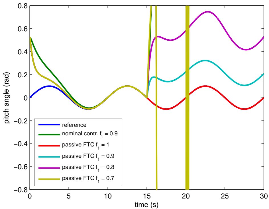
FIGURE 7.3: Pitch angle response (comparison between the nominal controller and the passive FTC).
