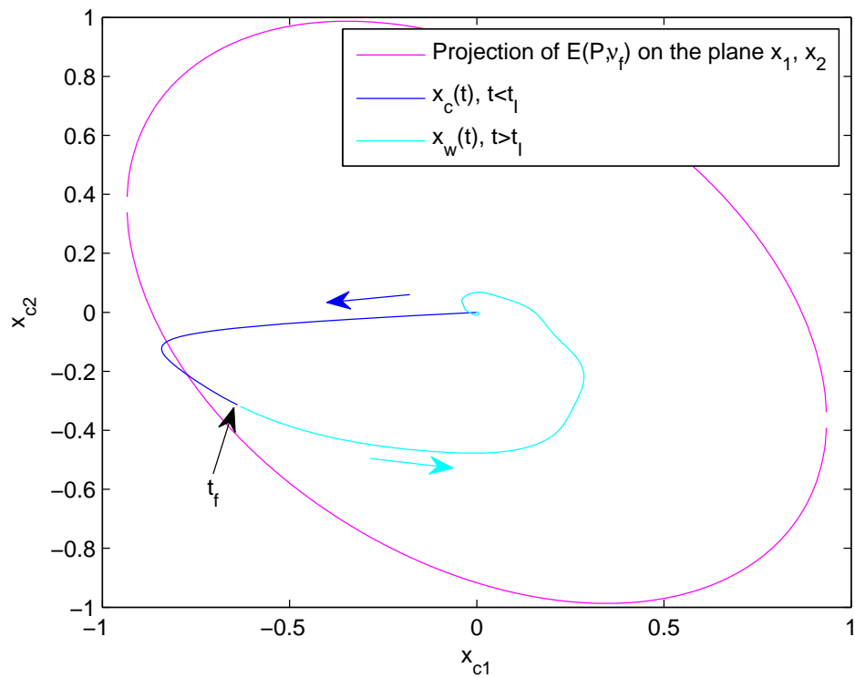
FIGURE 9.6: Phase plane of x_c(t) , t_f = t_I = 0.5 s.
