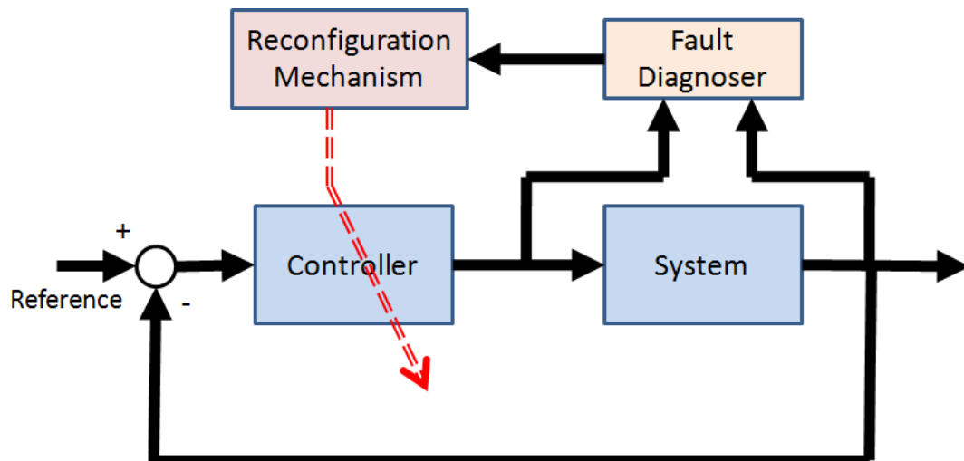
FIGURE 6.3: Active fault tolerant control conceptual scheme.
