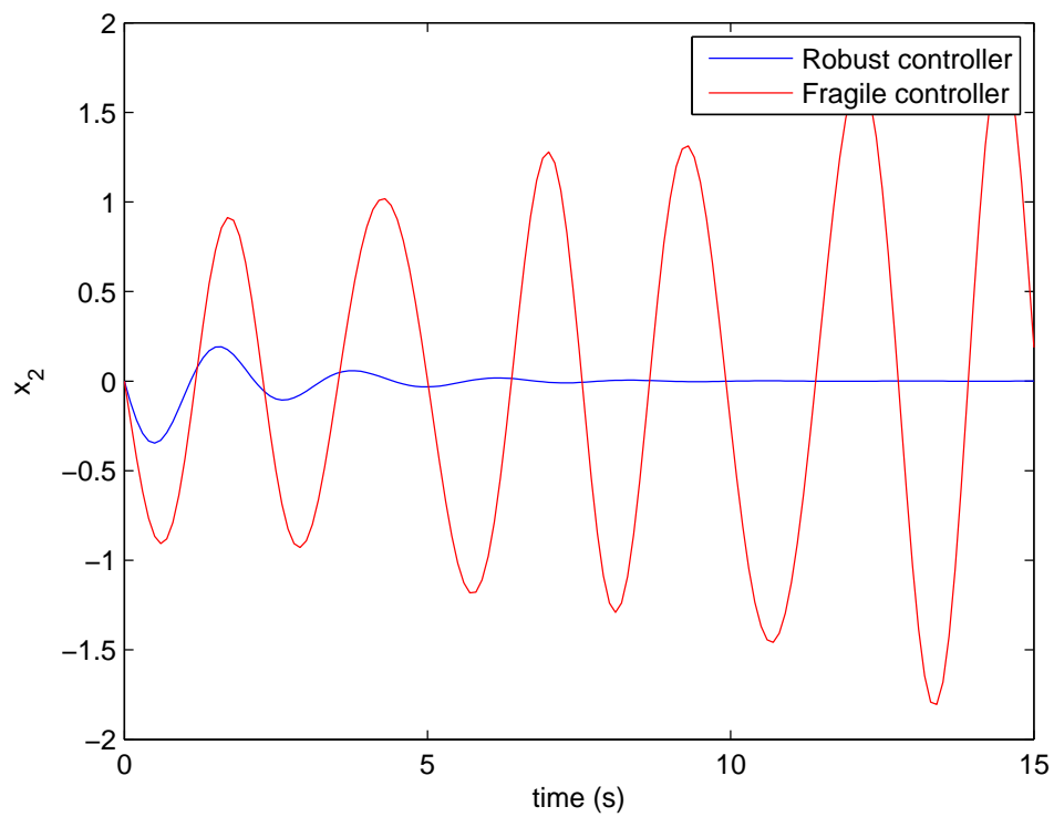
FIGURE 4.5: Robust \mathcal{D} -stability: closed-loop response of x_2(t) .
