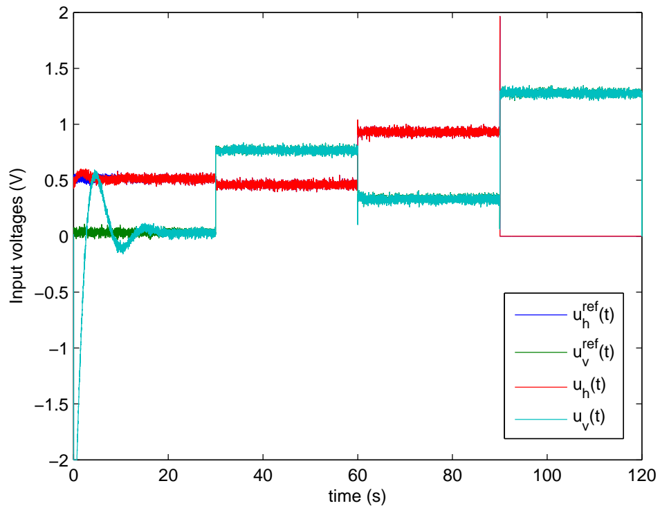
FIGURE 8.15: Faulty control inputs (with FTC).
