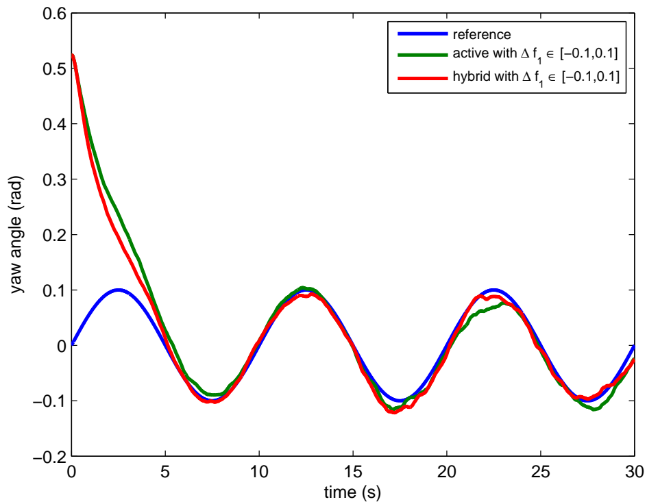
FIGURE 7.12: Yaw angle response (comparison between the active FTC and the hybrid FTC, f_1 = 0.7 ).
