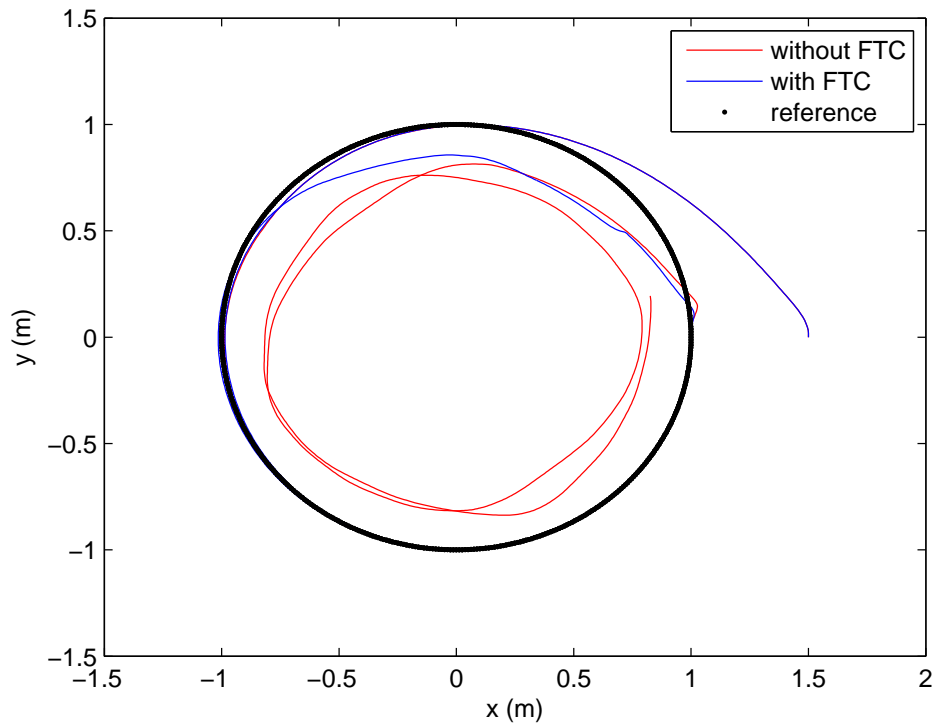
FIGURE 8.22: Tracking of the desired circular trajectory: (x - y) plane (Simulation 1).
