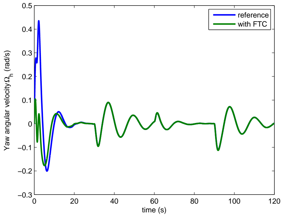
FIGURE 8.11: Faulty yaw angular velocity response (comparison between TRMS and reference model states, with FTC).
