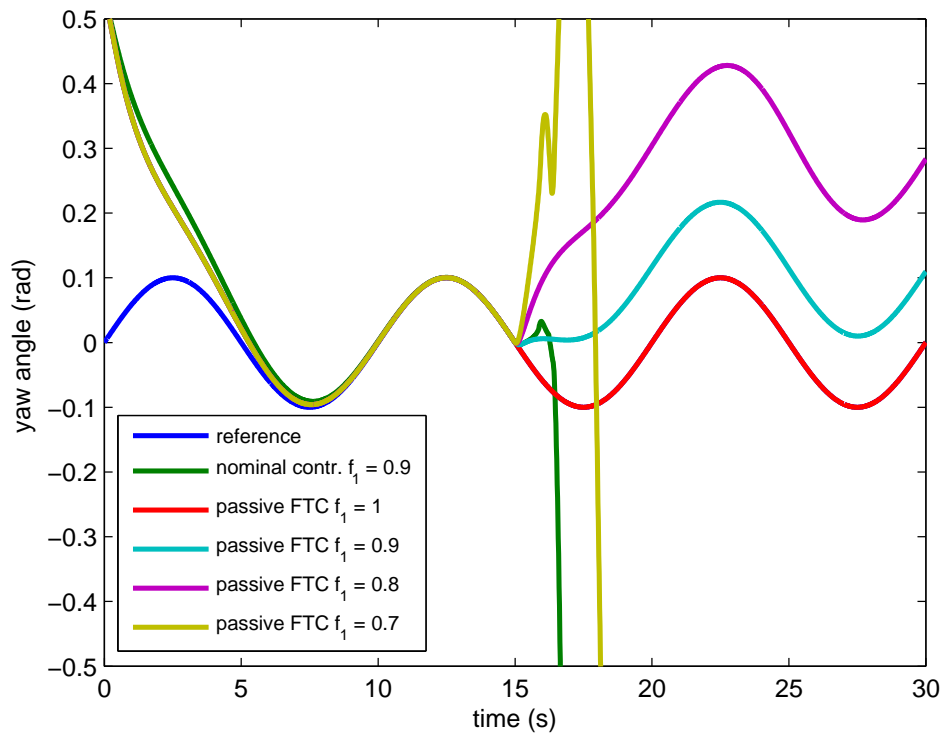
FIGURE 7.4: Yaw angle response (comparison between the nominal controller and the passive FTC).
