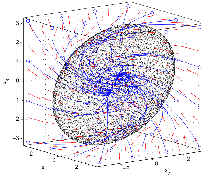
FIGURE 3.8: Trajectories and estimated region of attraction for the closed-loop system obtained using the model generated via sector nonlinearity concept.
