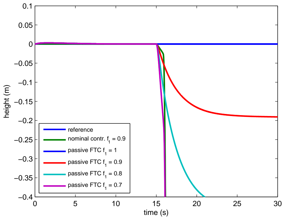
FIGURE 7.5: Height response (comparison between the nominal controller and the passive FTC).
