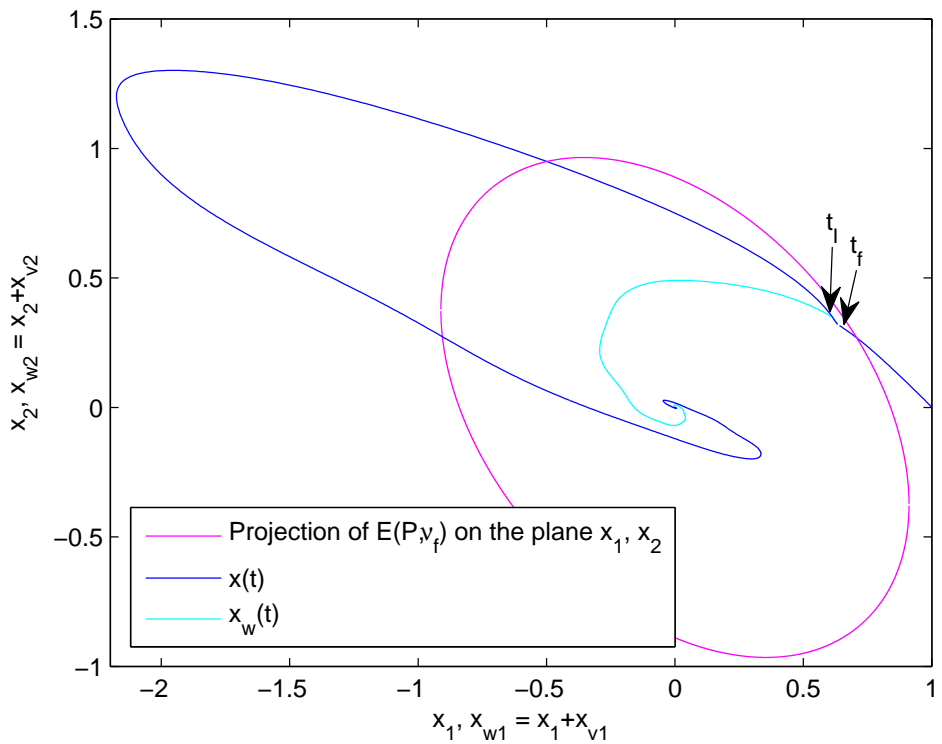
FIGURE 9.8: Phase plane of x(t) and x_w(t) , t_f = 0.5 s, t_I = 0.525 s.
