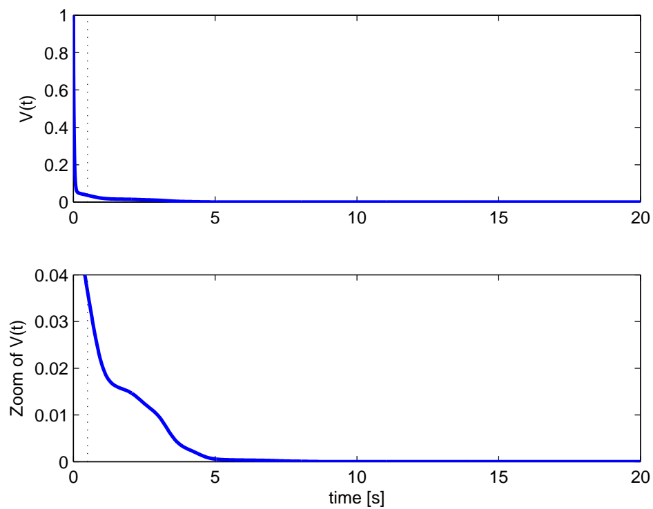
FIGURE 9.4: Lyapunov function V(t) , t_f = t_I = 0.5 s.
