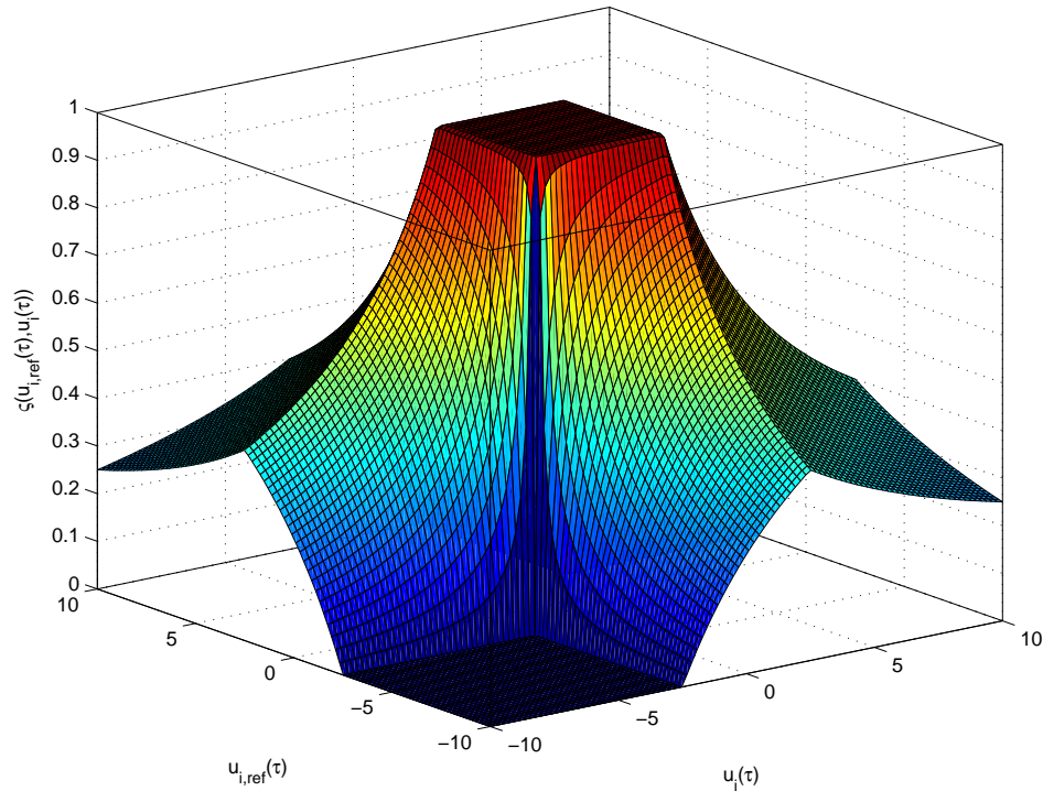
FIGURE 8.2: Graphical representation of \varsigma_i(u_{i,ref}(\tau), u_i(\tau)) with u_i^{MAX} = 2.5 .
