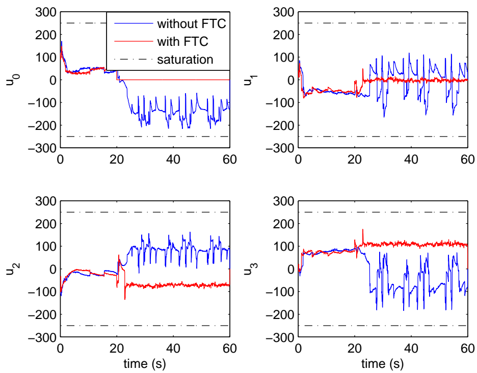
FIGURE 8.25: Tracking of the desired circular trajectory: inputs (Experiment 1)
