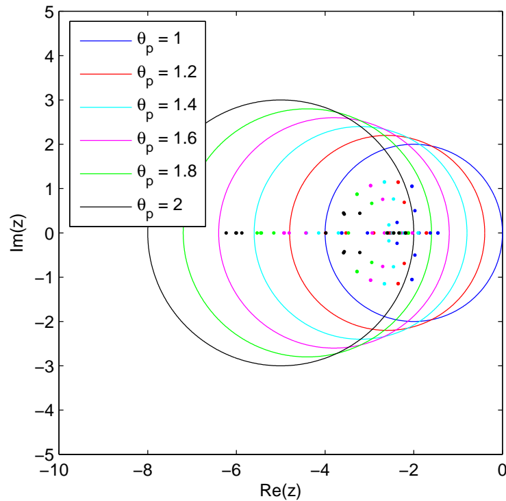
FIGURE 5.1: Shifting \mathcal{D} -stability: closed-loop poles.
