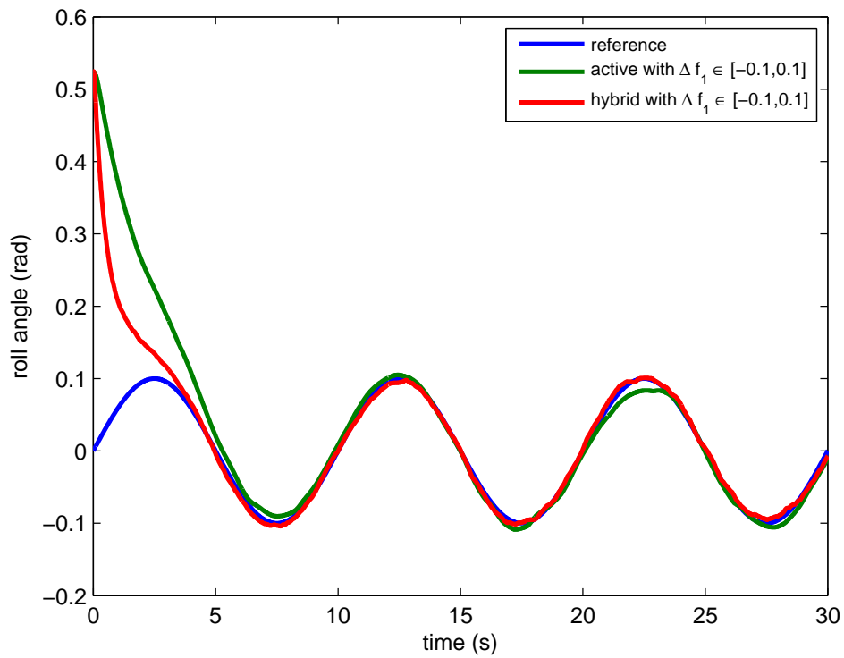
FIGURE 7.10: Roll angle response (comparison between the active FTC and the hybrid FTC, f_1 = 0.7 ).
