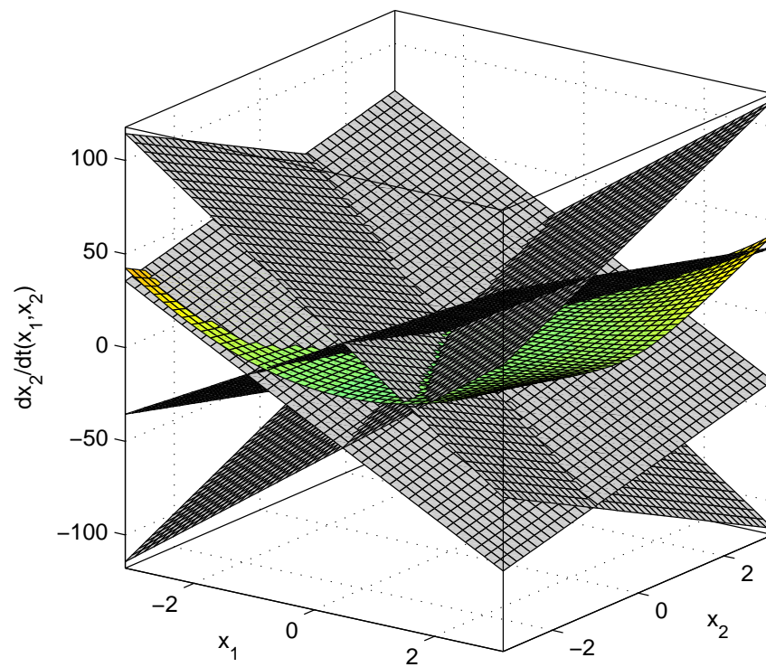
FIGURE 3.5: Representation of the nonlinear equation \dot{x}_2 = x_1^2 \sqrt{1 + x_2^2} + x_1 x_2 in \mathcal{P} and its approximation using the vertex systems of (3.56).
