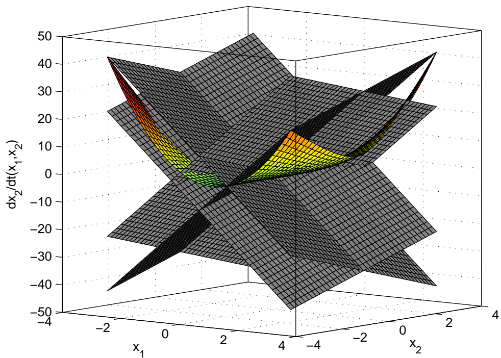
FIGURE 3.3: Representation of the nonlinear equation \dot{x}_2 = x_1^2 \sqrt{1+x_2^2} + x_1 x_2 in \mathcal{P} and its approximation using the subsystems described by A_i^{(4)} .
