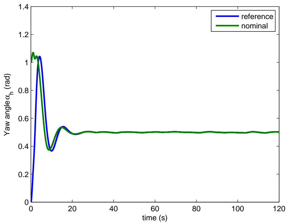
FIGURE 8.6: Nominal yaw angle response (comparison between TRMS and reference model states).
