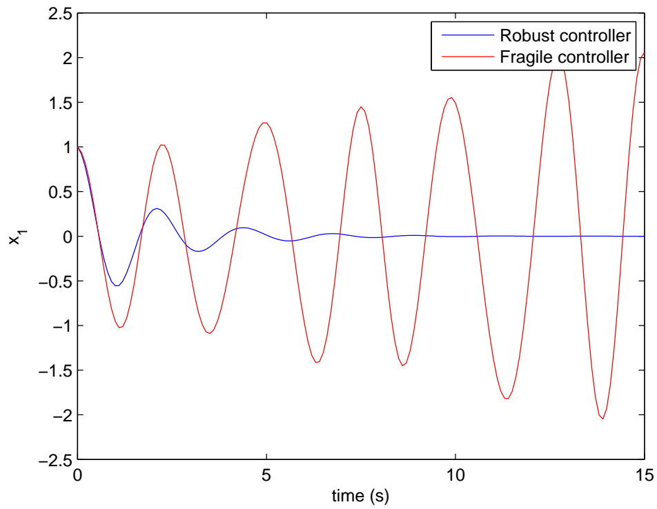
FIGURE 4.4: Robust \mathcal{D} -stability: closed-loop response of x_1(t) .
