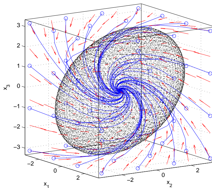
FIGURE 3.7: Trajectories and estimated region of attraction for the closed-loop system obtained using the model generated via nonlinear embedding with matrices A_i^{(4)} .
