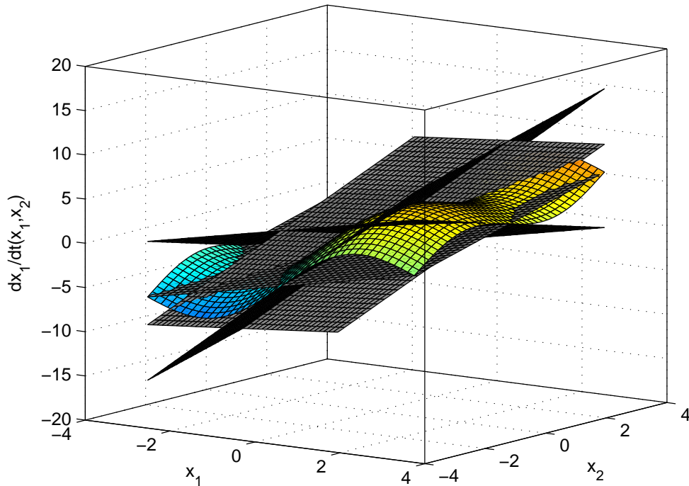
FIGURE 3.1: Representation of the nonlinear equation \dot{x}_1 = x_1 + 3 \sin x_1 + x_2 - 2 \sin x_2 in \mathcal{P} and its approximation using the subsystems described by A_i^{(3)} or A_i^{(4)} .
