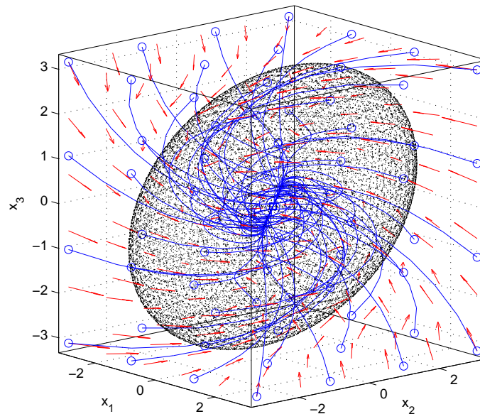
FIGURE 3.9: Trajectories and estimated region of attraction for the closed-loop system obtained using the model generated via sector nonlinearity concept (conservative).
