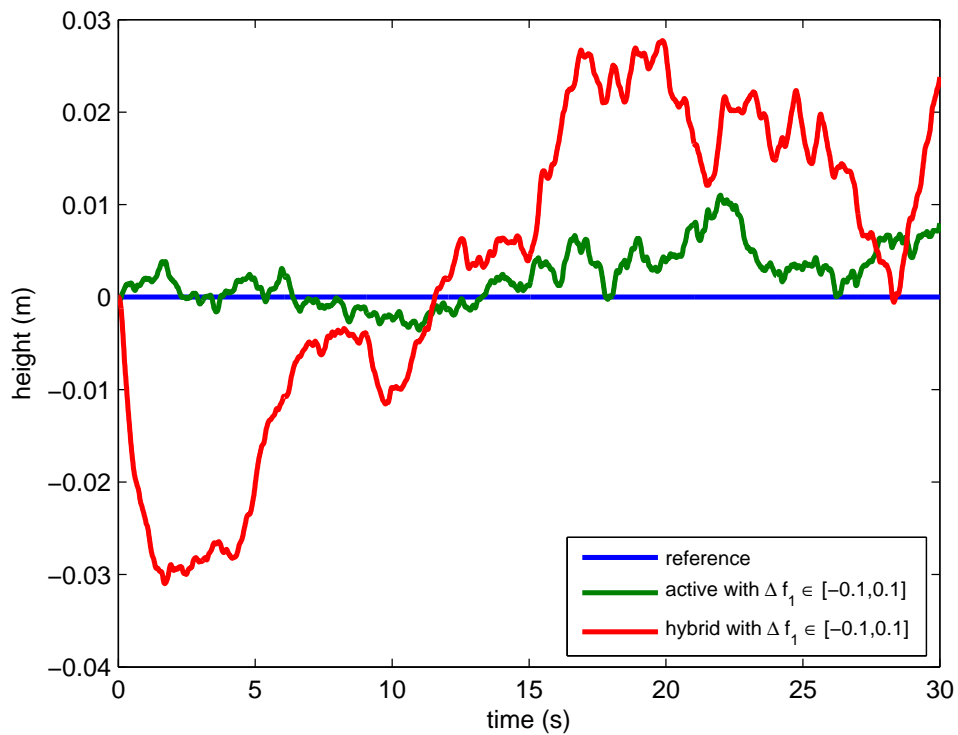
FIGURE 7.13: Height response (comparison between the active FTC and the hybrid FTC, f_1 = 0.7 ).
