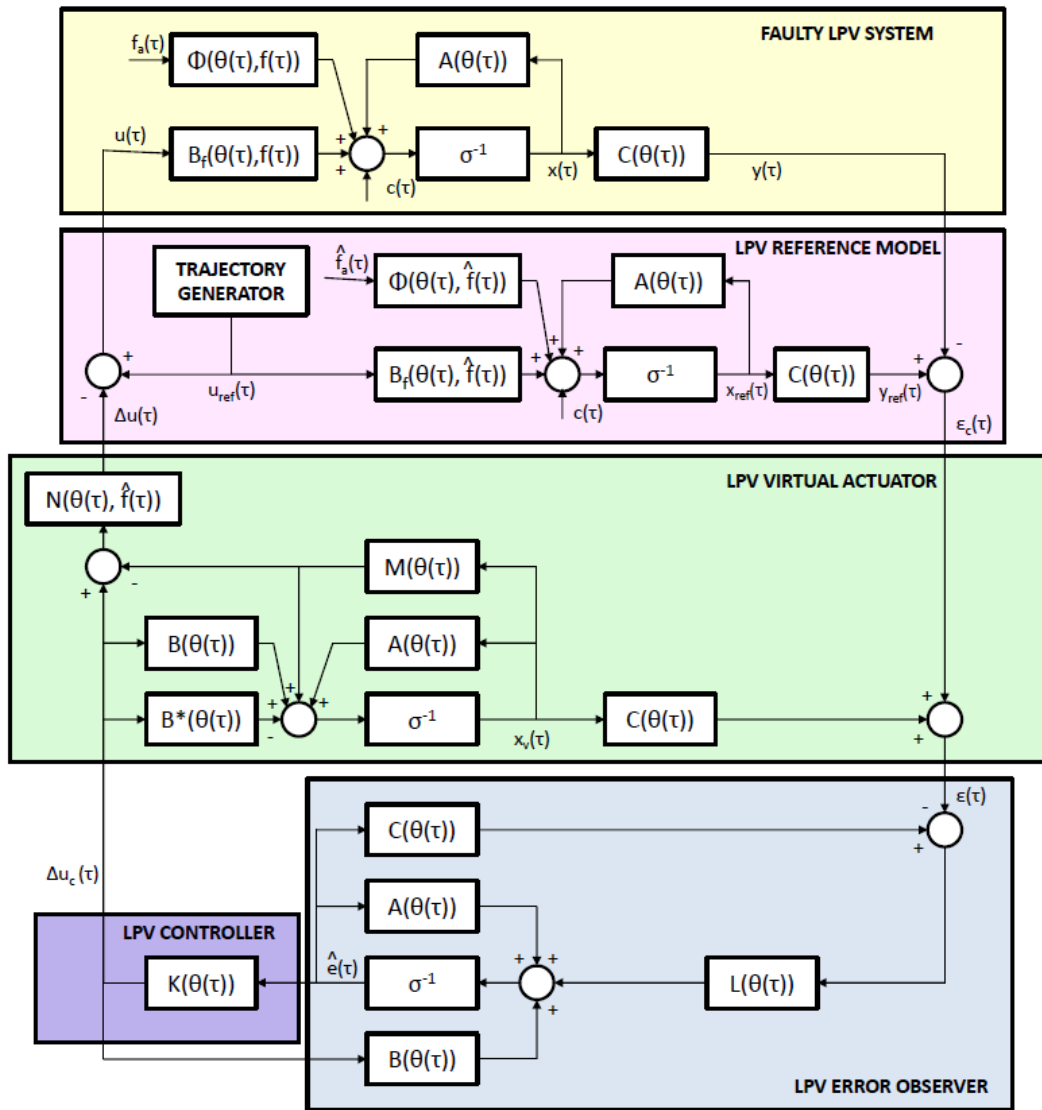
FIGURE 8.1: Virtual actuator FTC scheme.
