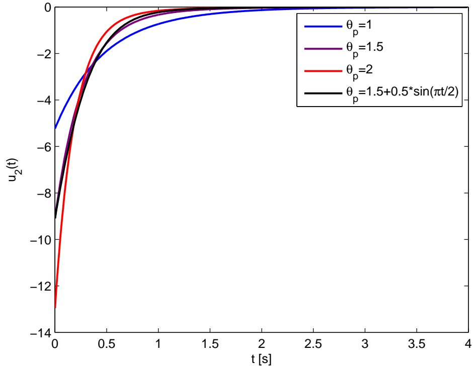
FIGURE 5.7: Shifting \mathcal{D} -stability: input signal u_2(t) .
