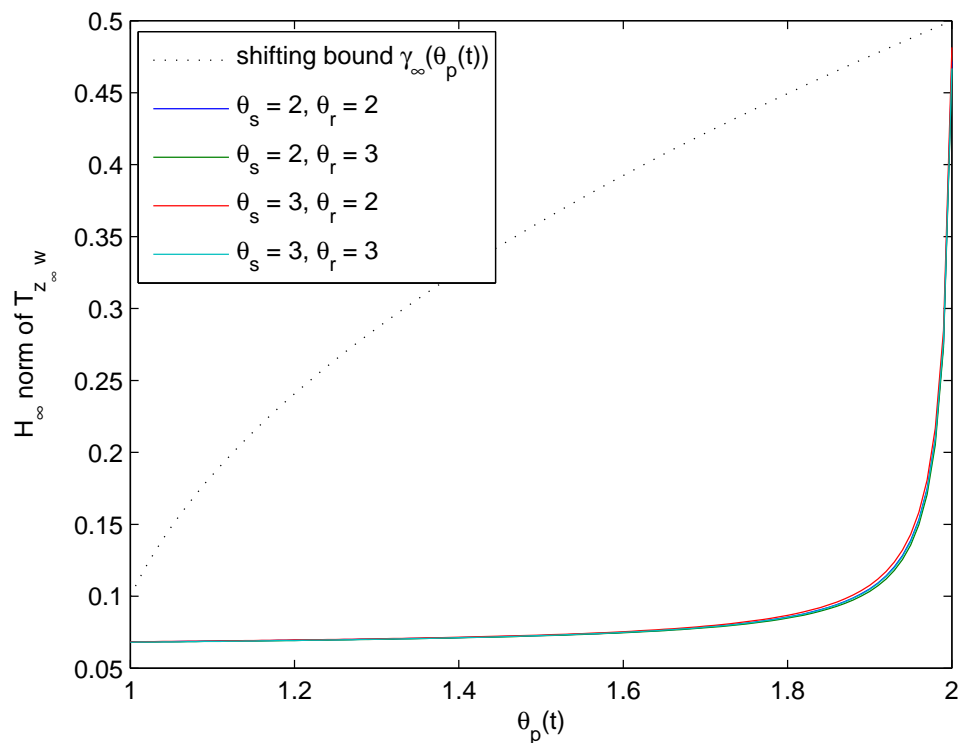
FIGURE 5.8: Shifting \mathcal{H}_\infty performance: bound on the \mathcal{H}_\infty norm.
