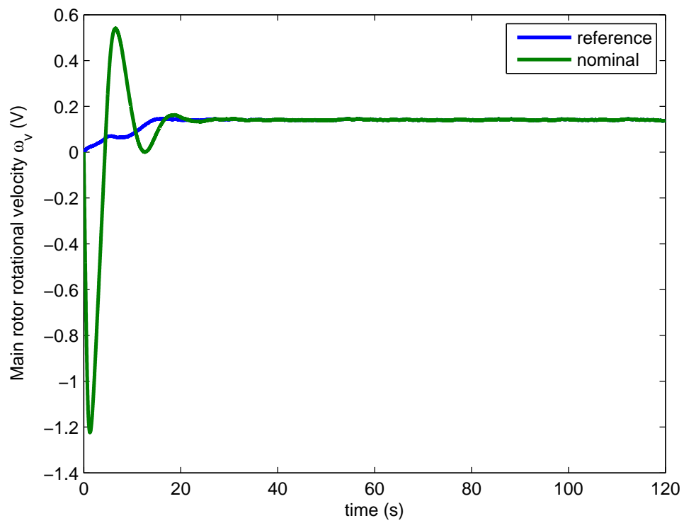
FIGURE 8.7: Nominal main rotor response (comparison between TRMS and reference model states).
