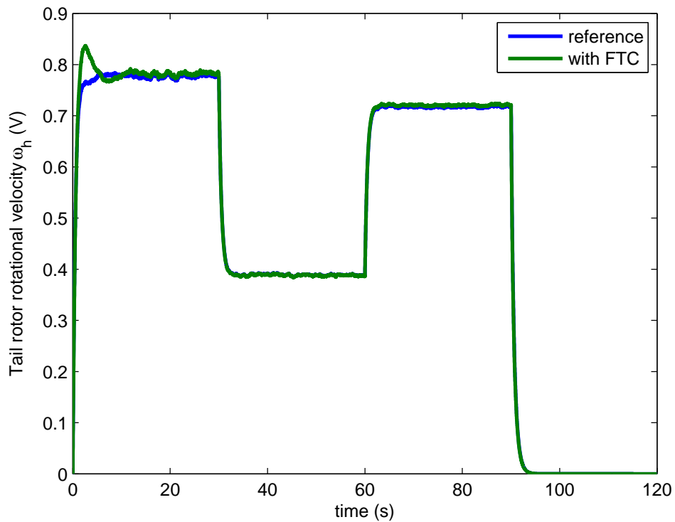
FIGURE 8.10: Faulty tail rotor response (comparison between TRMS and reference model states, with FTC).
