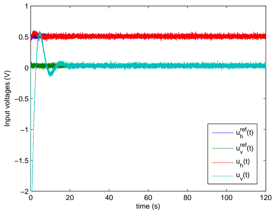
FIGURE 8.9: Nominal control inputs.
