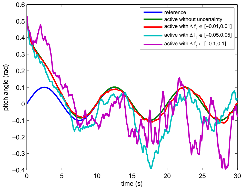
FIGURE 7.7: Pitch angle response (active FTC without and with uncertainty, f_1 = 0.7 ).
