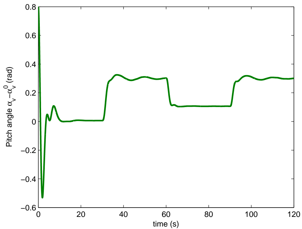
FIGURE 8.14: Faulty pitch angle response (with FTC).
