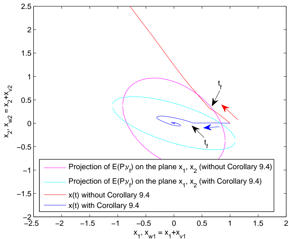
FIGURE 9.9: Comparison between the state trajectories obtained with the controllers designed using Corollary 9.1 and Corollary 9.4 ( \lambda = 0 , t_f = 0.5 s), respectively, when no fault isolation is performed during the simulation.
