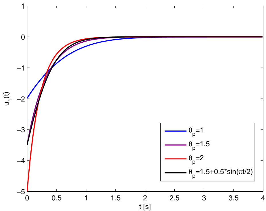
FIGURE 5.6: Shifting \mathcal{D} -stability: input signal u_1(t) .
