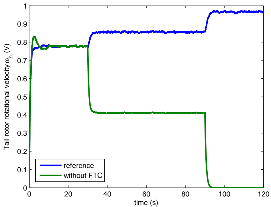
FIGURE 8.16: Faulty tail rotor response (comparison between TRMS and reference model states, without FTC).
