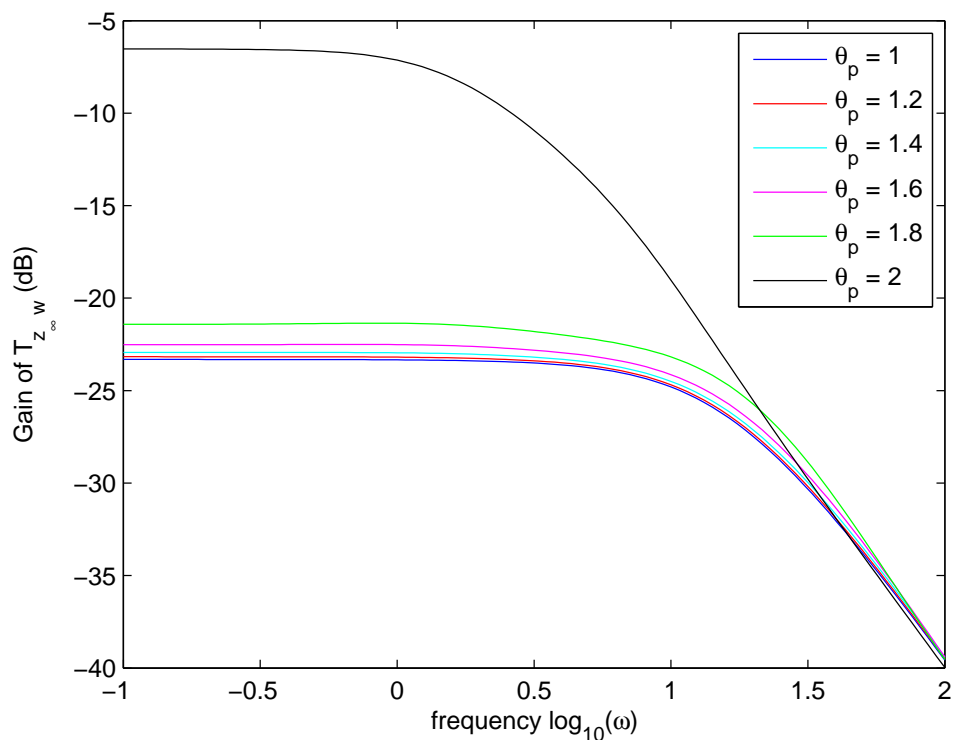
FIGURE 5.9: Shifting \mathcal{H}_\infty performance: variation of the Bode plot according to changes in \theta_p , obtained for \theta_s = \theta_r = 2 .
