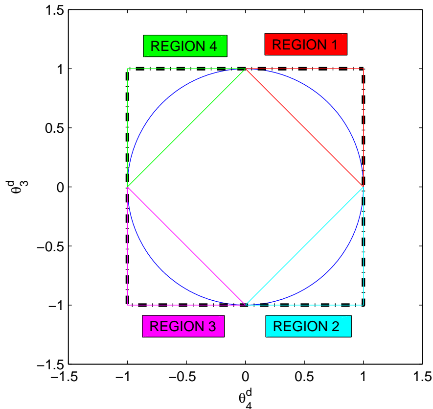
FIGURE 8.21: Polytopic LPV and polytopic switching LPV approximations of the scheduling variables \theta_3^d(k) and \theta_4^d(k) .
