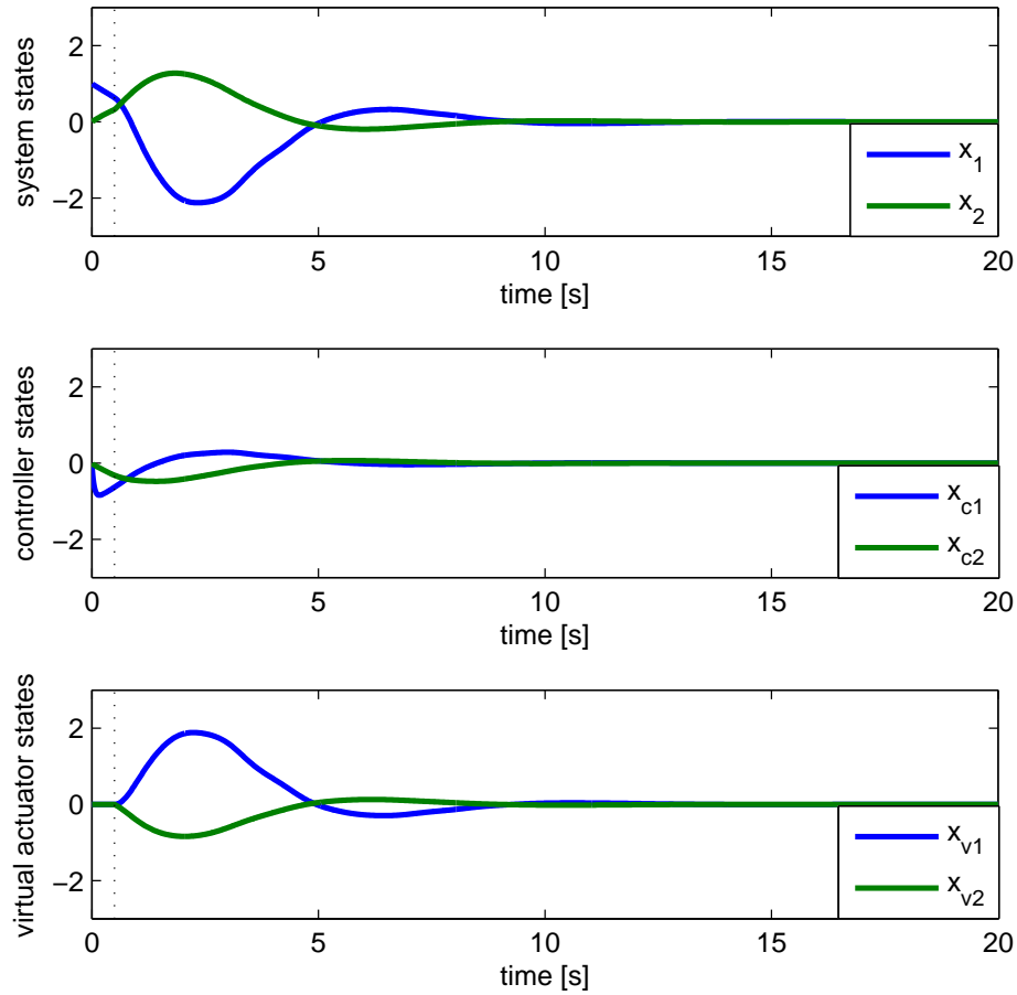
FIGURE 9.2: State trajectory, t_f = t_I = 0.5 s.
