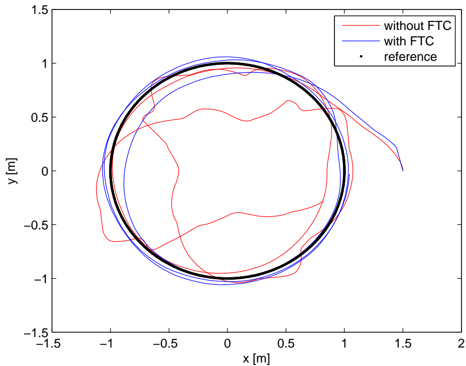
FIGURE 8.23: Tracking of the desired circular trajectory: (x - y) plane (Experiment 1)
