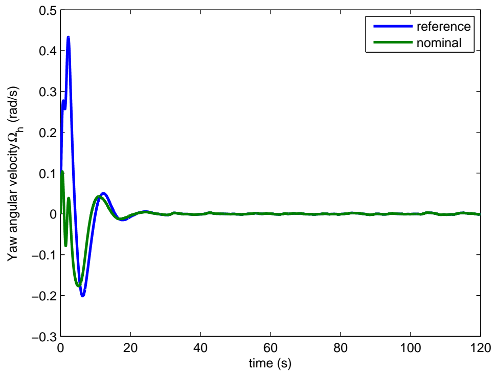
FIGURE 8.5: Nominal yaw angular velocity response (comparison between TRMS and reference model states).
