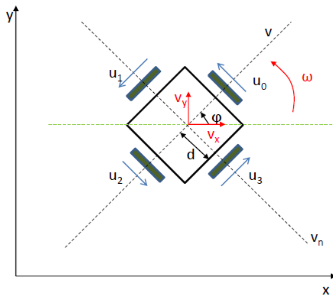
FIGURE 8.20: Four wheeled omnidirectional mobile robot.
