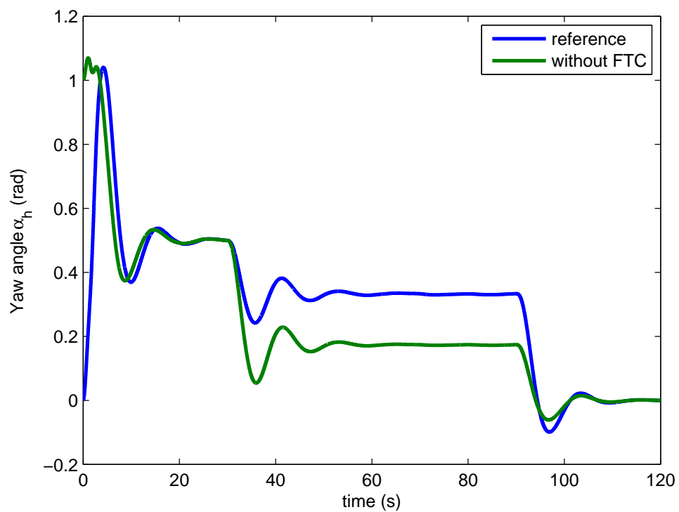
FIGURE 8.18: Faulty yaw angle response (comparison between TRMS and reference model states, without FTC).
