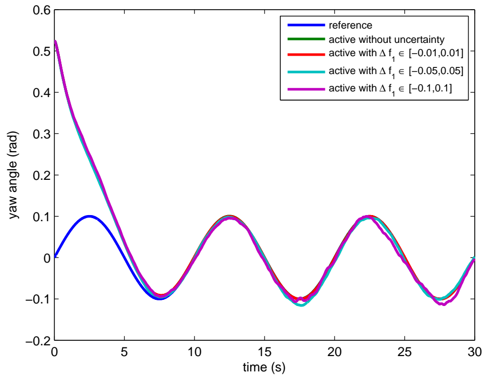
FIGURE 7.8: Yaw angle response (active FTC without and with uncertainty, f_1 = 0.7 ).
