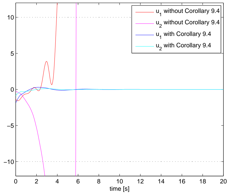
FIGURE 9.10: Control inputs with and without applying Corollary 9.4, t_f = 0.5 s, and no fault isolation during the simulation ( t_I > 20 s).
