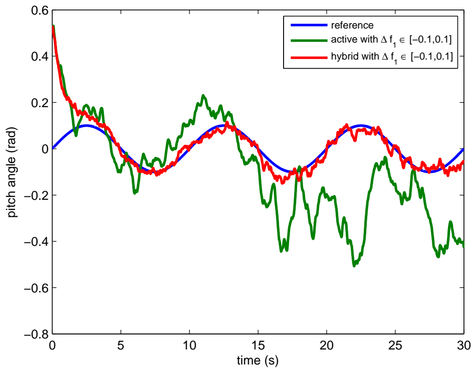
FIGURE 7.11: Pitch angle response (comparison between the active FTC and the hybrid FTC, f_1 = 0.7 ).
