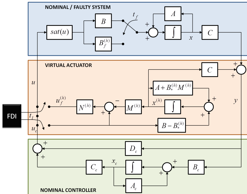
FIGURE 9.1: Overall fault tolerant control scheme.
