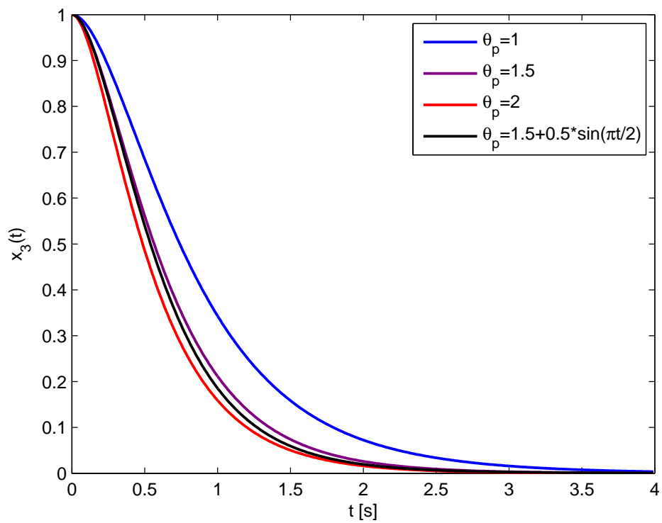
FIGURE 5.4: Shifting \mathcal{D} -stability: closed-loop response of x_3(t) .
