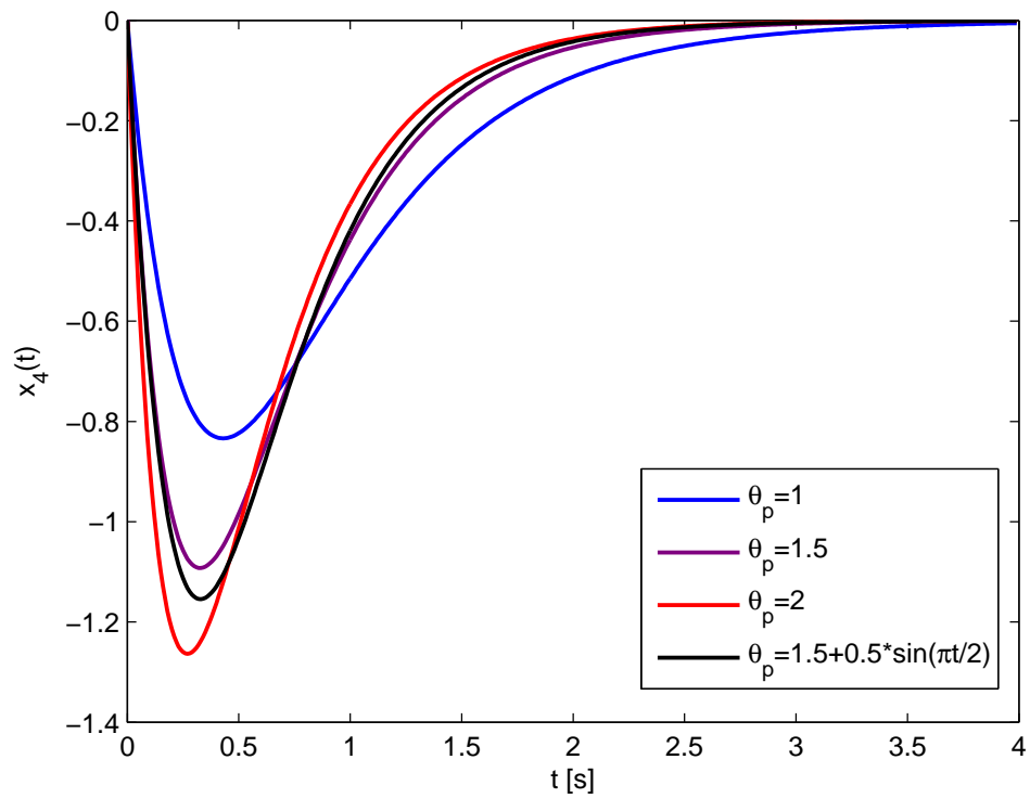
FIGURE 5.5: Shifting \mathcal{D} -stability: closed-loop response of x_4(t) .
