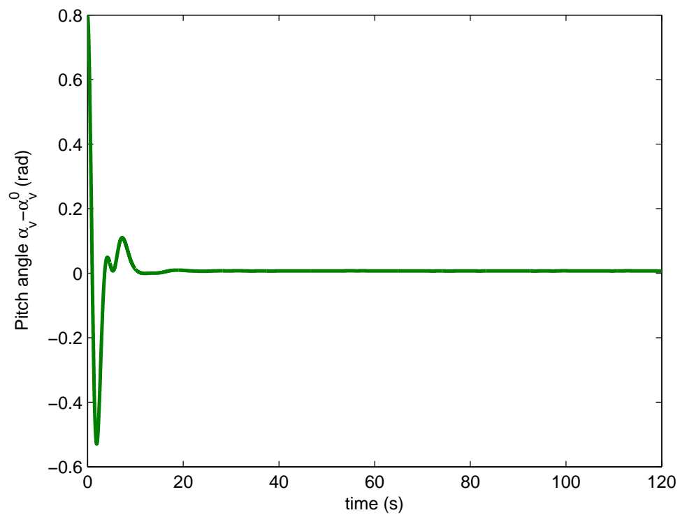
FIGURE 8.8: Nominal pitch angle response.
