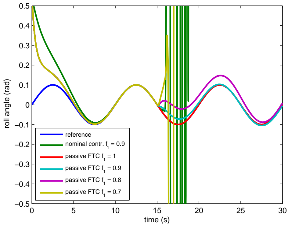
FIGURE 7.2: Roll angle response (comparison between the nominal controller and the passive FTC).
