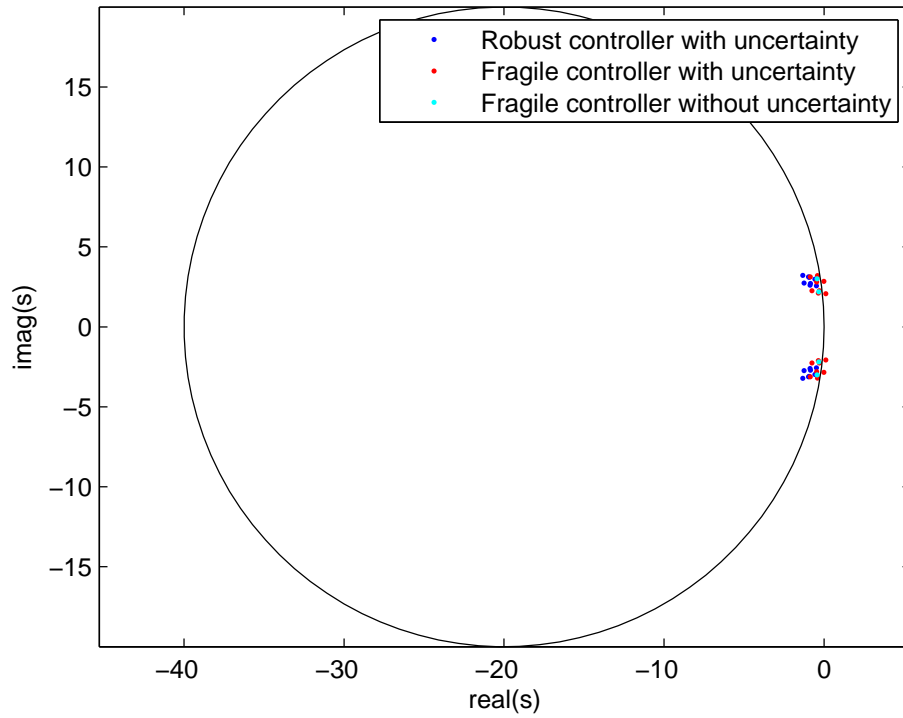
FIGURE 4.2: Robust \mathcal{D} -stability: comparison between robust and fragile controller.
