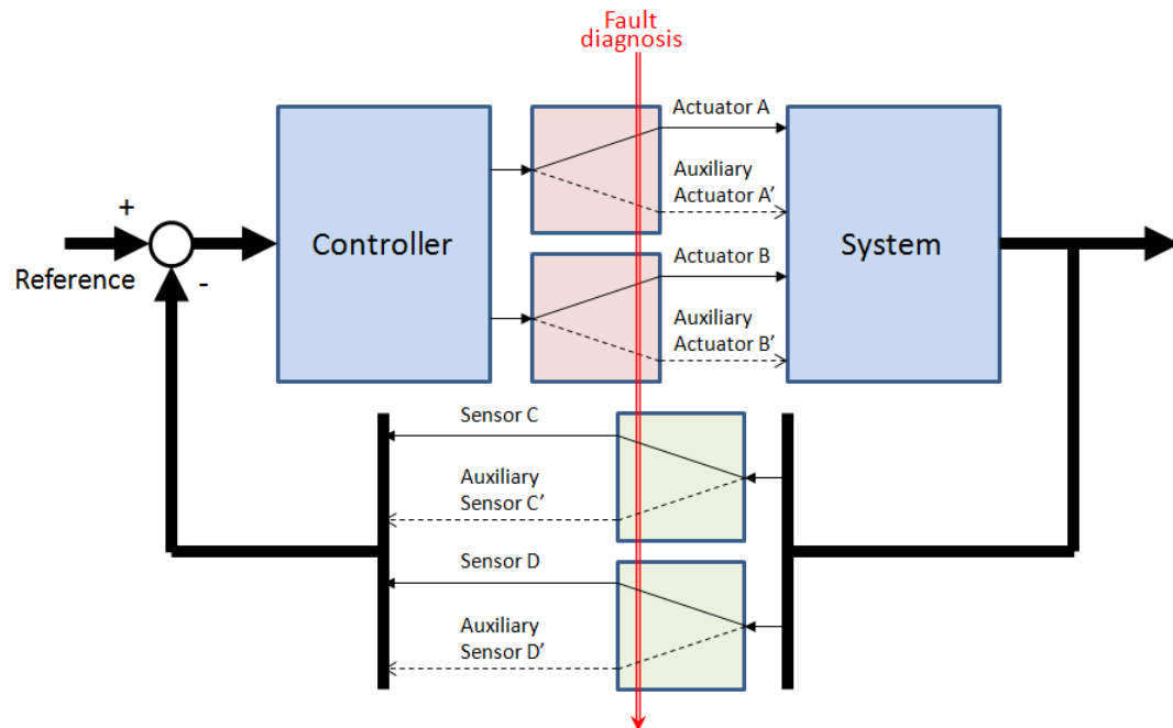
FIGURE 6.1: Hardware redundancy conceptual scheme.
