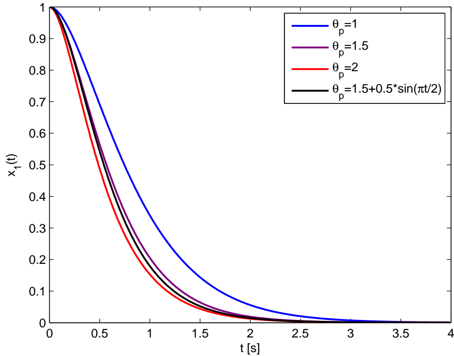
FIGURE 5.2: Shifting \mathcal{D} -stability: closed-loop response of x_1(t) .
