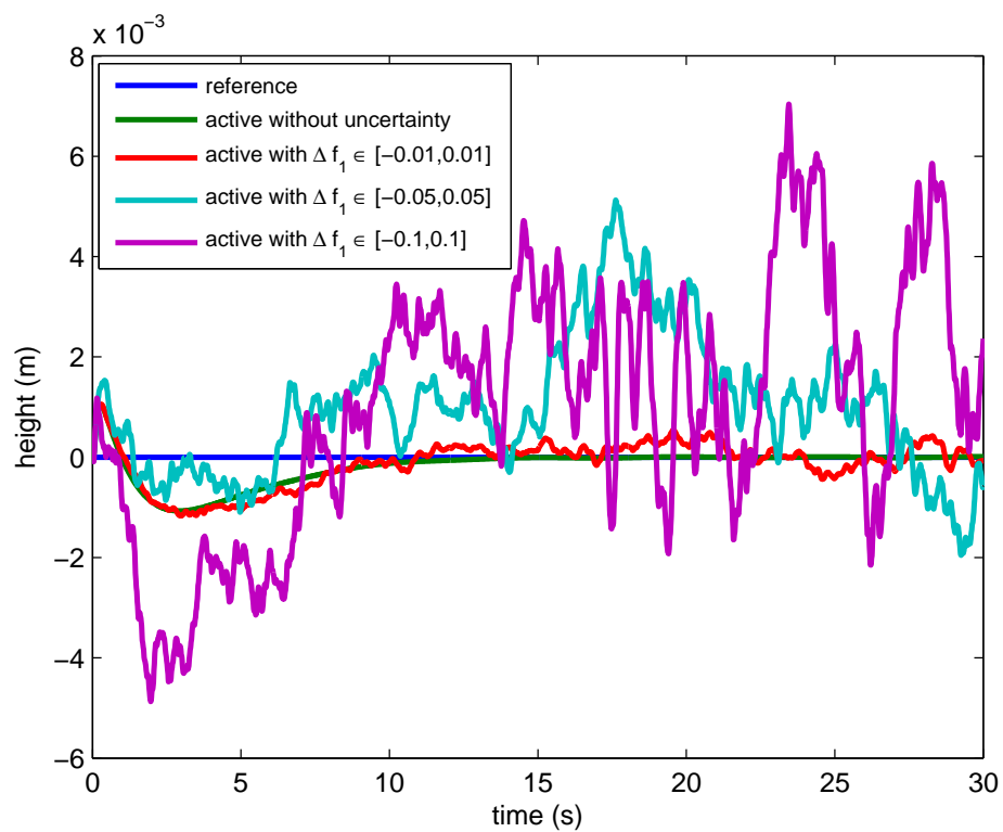
FIGURE 7.9: Height response (active FTC without and with uncertainty, f_1 = 0.7 ).
