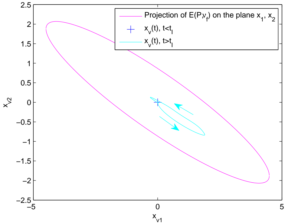
FIGURE 9.7: Phase plane of x_v(t) , t_f = t_I = 0.5 s.
