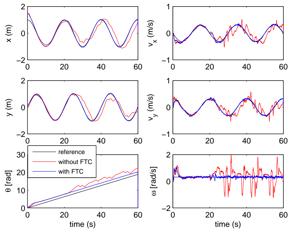
FIGURE 8.24: Tracking of the desired circular trajectory: states (Experiment 1)
