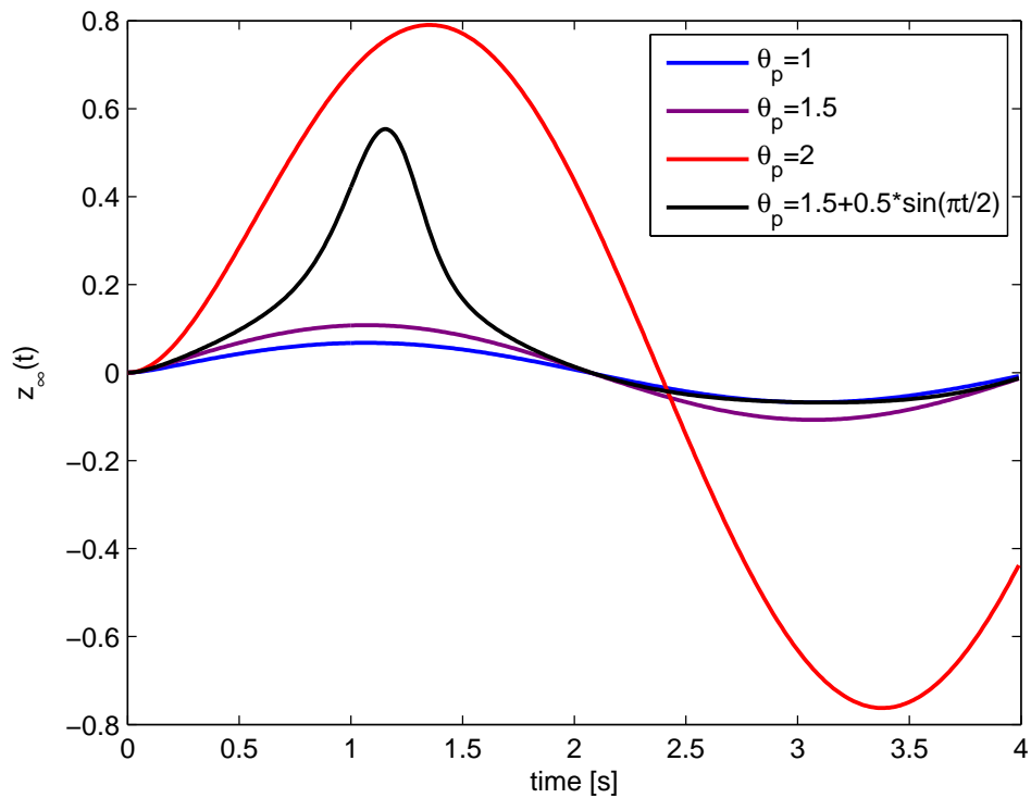
FIGURE 5.10: Shifting \mathcal{H}_\infty performance: response of the closed-loop system to an exogenous input w = \sin(t) .
