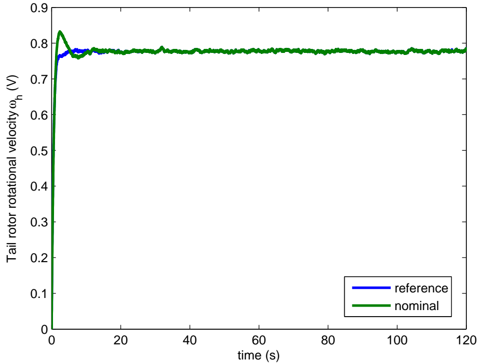
FIGURE 8.4: Nominal tail rotor response (comparison between TRMS and reference model states).
