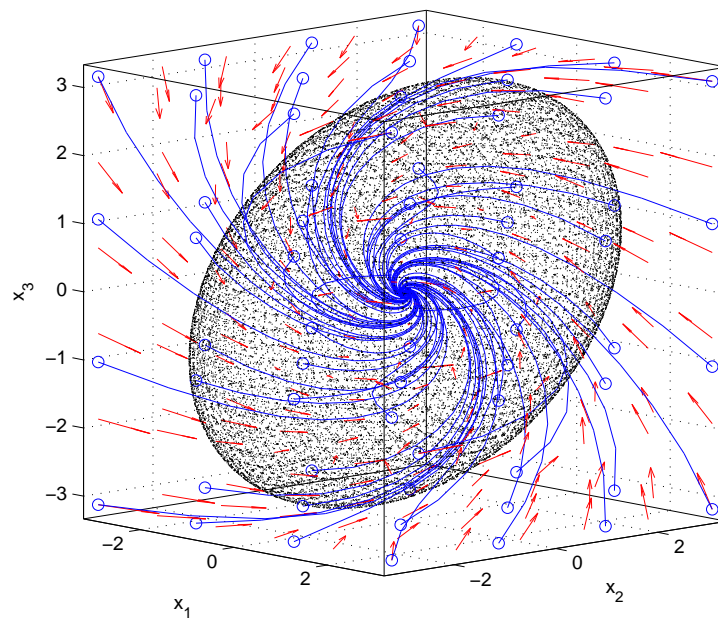
FIGURE 3.6: Trajectories and estimated region of attraction for the closed-loop system obtained using the model generated via nonlinear embedding with matrices A_i^{(3)} .
