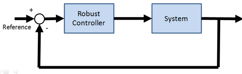
FIGURE 6.2: Passive fault tolerant control conceptual scheme.
