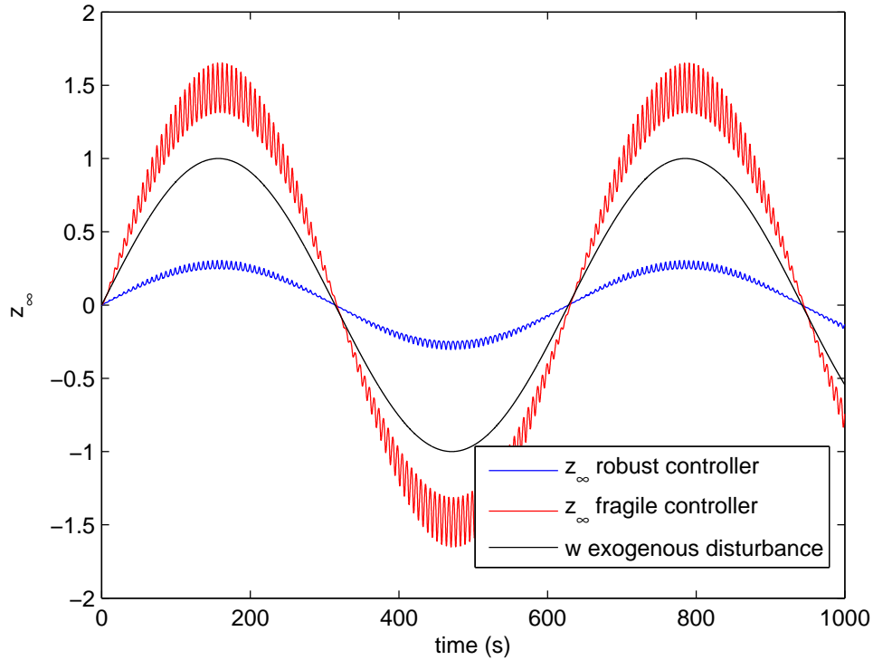
FIGURE 4.7: Robust \mathcal{H}_\infty performance: closed-loop response of z_\infty(t) .
