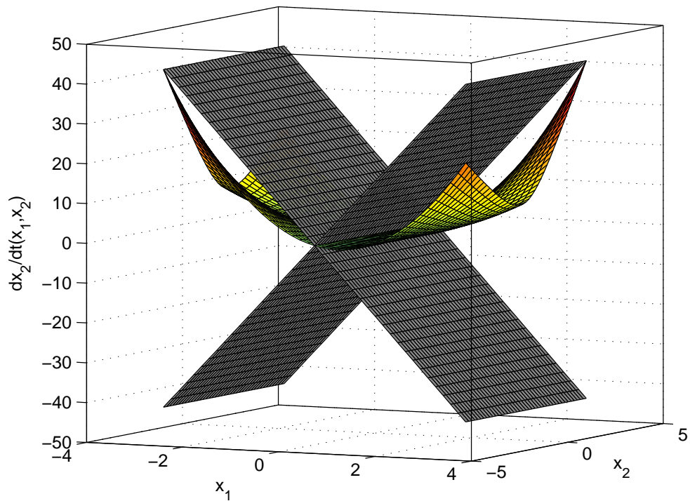
FIGURE 3.2: Representation of the nonlinear equation \dot{x}_2 = x_1^2 \sqrt{1+x_2^2} + x_1 x_2 in \mathcal{P} and its approximation using the subsystems described by A_i^{(3)} .
