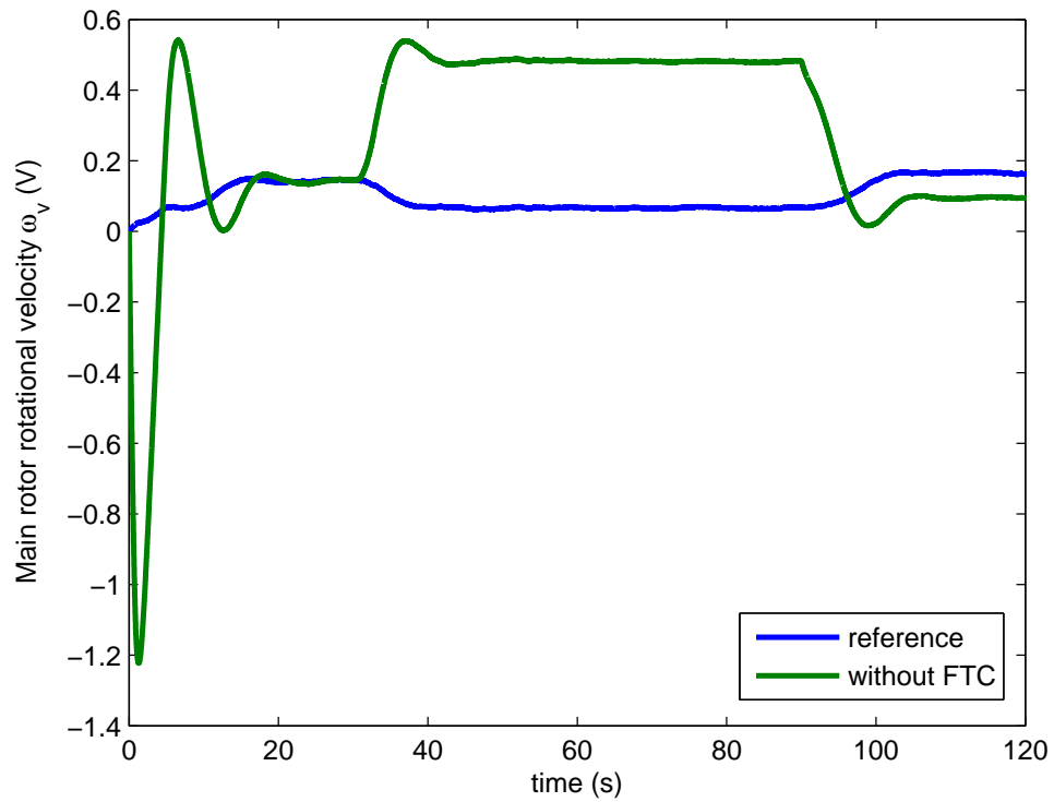
FIGURE 8.19: Faulty main rotor response (comparison between TRMS and reference model states, without FTC).
