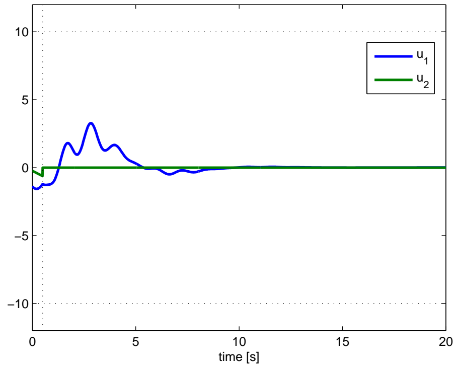
FIGURE 9.3: Control inputs, t_f = t_I = 0.5 s.
