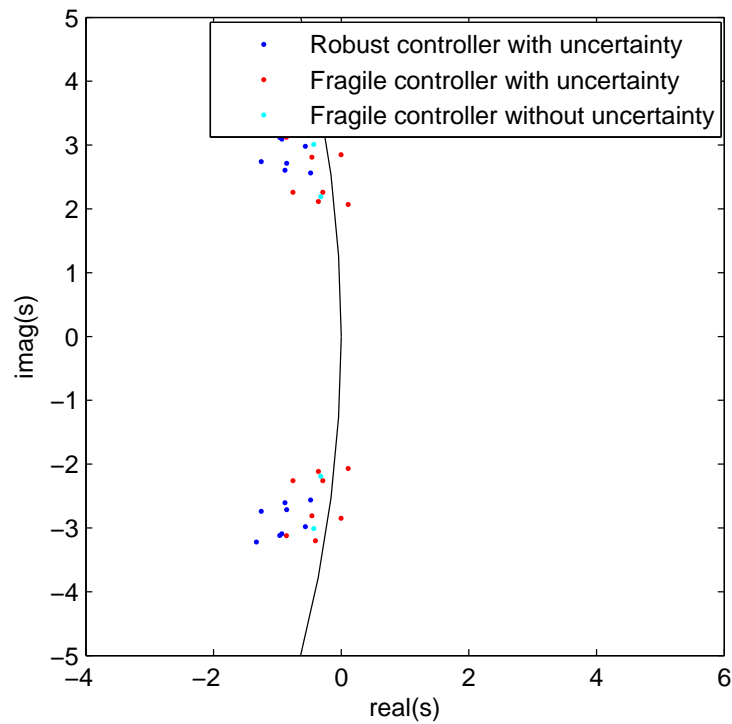
FIGURE 4.3: Robust \mathcal{D} -stability: comparison between robust and fragile controller (zoom).
