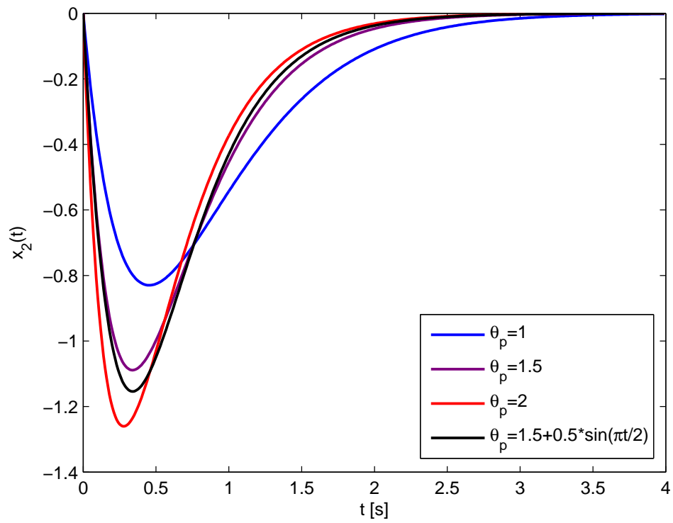
FIGURE 5.3: Shifting \mathcal{D} -stability: closed-loop response of x_2(t) .
