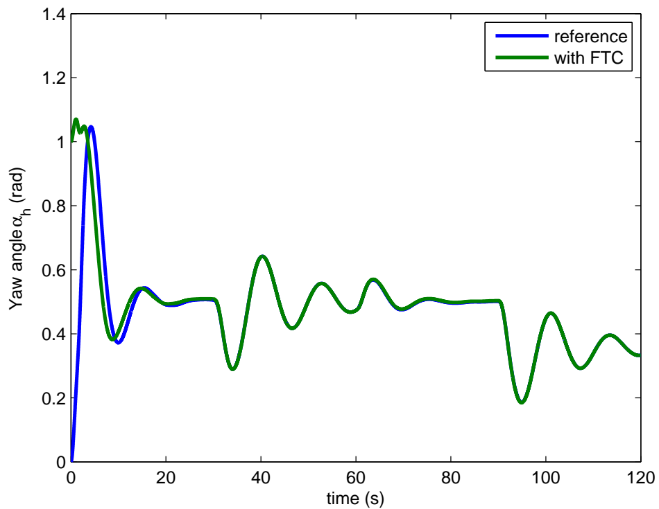
FIGURE 8.12: Faulty yaw angle response (comparison between TRMS and reference model states, with FTC).
