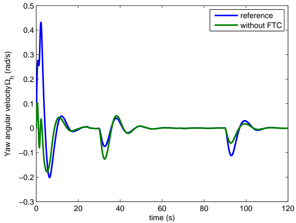
FIGURE 8.17: Faulty yaw angular velocity response (comparison between TRMS and reference model states, without FTC).
