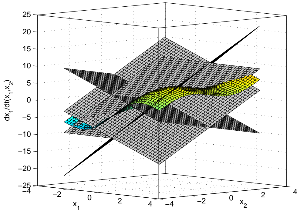
FIGURE 3.4: Representation of the nonlinear equation \dot{x}_1 = x_1 + 3 \sin x_1 + x_2 - 2 \sin x_2 in \mathcal{P} and its approximation using the vertex systems of (3.56).
