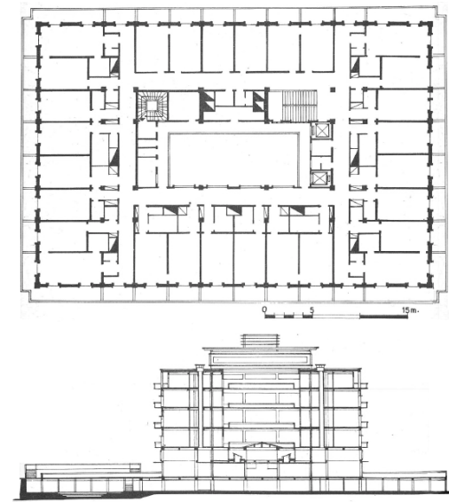
6 | 1931. Hotel Saint Georges. Beirut. Jacques Poirrier, Georges Bordes y Andre Lotte Arab Center for Architecture [o] [c: 09.02.20] [d]: http://www.arab-architecture.org/db/building/hotel-saint-georges-1 || Saint-George Hotel [o] [c: 09.02.20] [d]: http://saintgeorgebeirut.com/
