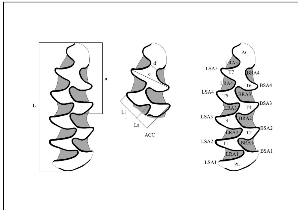
Figure 1. Nomenclature and measurement methods used for m1 in the description of arvicoline. L : total length; a : length of the anteroconid complex; e : width of the anteroconid complex; d : degree of closure of AC; La : width of T4; Li : width of T5; PL : posterior lobe; ACC : anteroconid complex; AC : anterior cap; BRA : buccal reentrant angle; BSA : buccal salient angle; LRA : lingual reentrant angle; LSA : lingual salient angle; T1-T7 : triangles 1-7.
