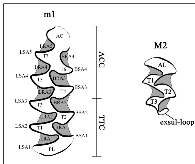
Figure 1.3.1. Nomenclature for the description of the first lower molar (m1) and second upper molar (M2). AL: anterior lobe; PL: posterior lobe; T: triangle; AC: anterior cap; LSA: lingual salient angle; LRA: lingual reentrant angle; BSA: buccal salient angle; BRA: buccal reentrant angle. ACC: anteroconid complex; TTC: talonid-trigonid complex. After Van der Meulen (1973) and Nadachowski (1982).
