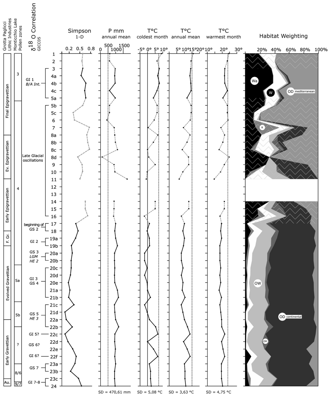
Fig. 4. Representation of the small mammal Simpson diversity index (1-D), the mean annual precipitation (MAP), the mean annual temperature of the coldest month (MTC), the mean annual temperature (MAT) the mean annual temperature of the warmest month (MTW) and the landscape percentages (OD mediterranean: open meadows related to Mediterranean conditions; OD continental: open meadows related to continental conditions; OH: open humid meadows; W: woodlands; R: rocky areas; Wa: areas along streams, lakes and ponds); Habitat Weighting white lines (from layer 16 to 5b, layers 3 and 2): low MNI.
