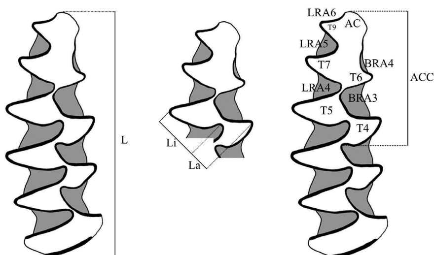
Figure 2. Nomenclature and measurement methods used for m1 in the description of arviculines.
