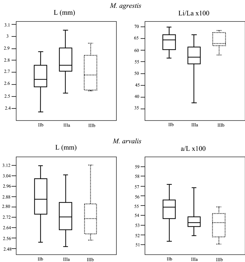
Fig. 2 Box plot showing significant measurements of M. agrestis (L and Li/La) and M. arvalis (L and a/L). Black lines : levels IIb and IIIa. Dotted lines : level IIIb (not statistically significant)
