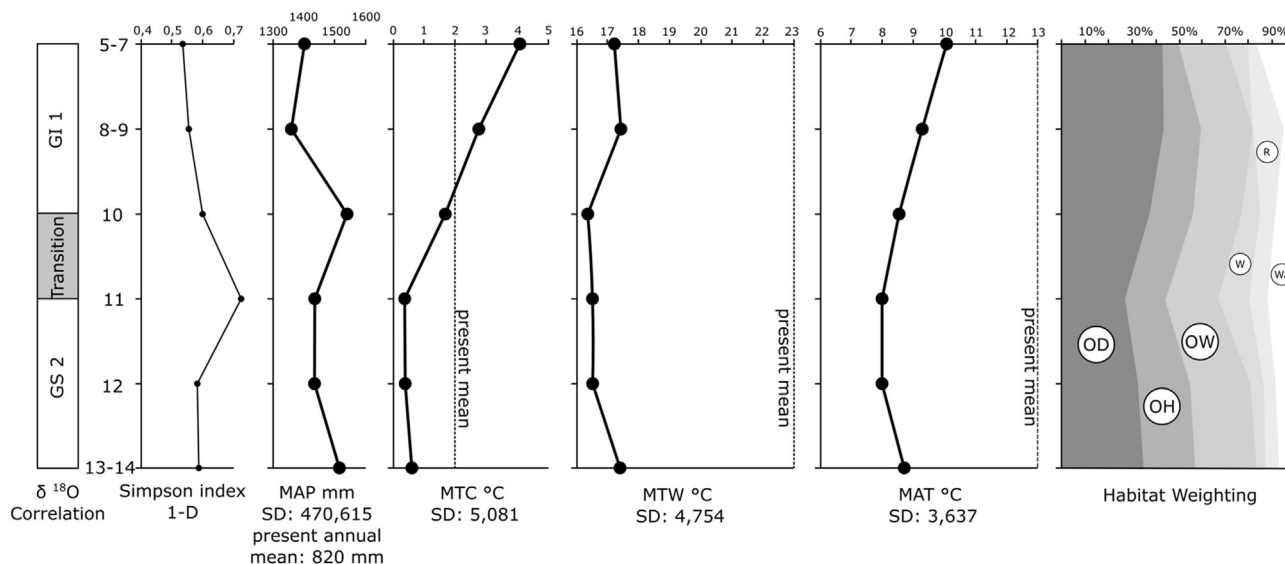
Fig. 4. Representation of the small mammal Simpson diversity index (1-D), the mean annual precipitation (MAP), the mean annual temperature of the coldest month (MTC), the mean annual temperature of the warmest month (MTW), the mean annual temperature (MAT), and the landscape percentages (OD: open dry meadows; OH: open humid meadows; OW: open woodland, woodland-edge; W: woodlands; R: rocky areas; Wa: areas along streams, lakes and ponds); SD: Standard Deviation, from Hernández Fernández (2001b).
