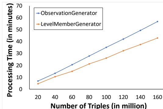
Fig. B.12: Scalability of LevelMemberGenerator and ObservationGenerator .
