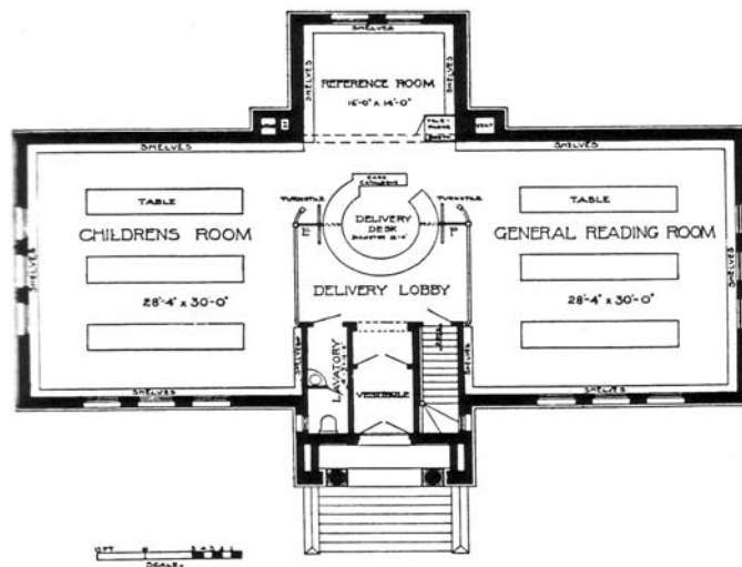
Figure 3.39 Carnegie Library of Pittsburgh, West End Branch, first-floor plan. Koch, Book of Carnegie Libraries (1917).
