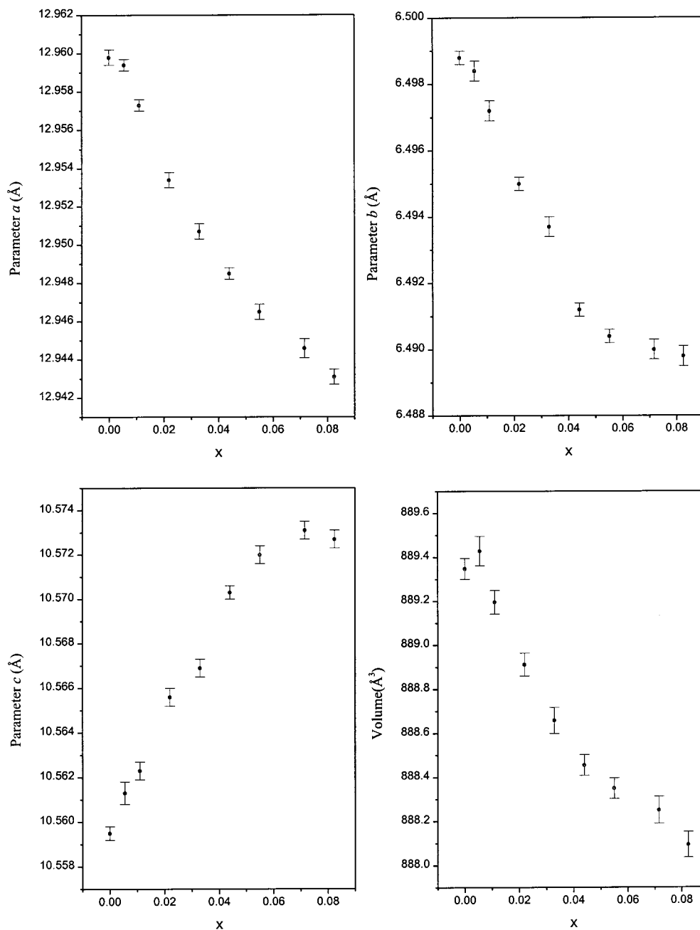
Figure 7. Evolution of the cell parameters and cell volume of the \text{RbTi}_{1-x}\text{Nb}_x\text{OPO}_4 crystals as a function of the concentration of niobium.
