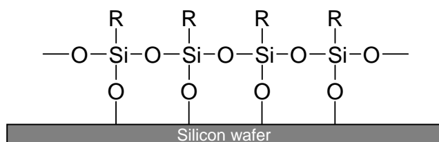
Figure 34. Scheme of a cross-linked silane monolayer.
